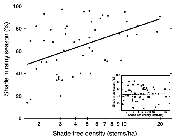
Fig. 3 Increased density of shade trees leads to greater shade during the rainy season (Shade = 40.7 + 36.9 log 10 (stems/ha), R^2_{adj} = 0.19 , F_{1,49} = 12.7 , P = 0.0008 ), but not during the dry season when many trees are deciduous (insert; R^2_{adj} = 0.02 , F_{1,49} = 0.79 , P = 0.71 )
