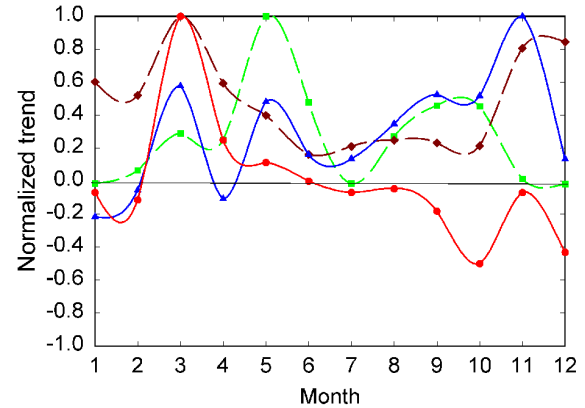
Figure 2: Normalized monthly trends (1950-1993) in continental average precipitation (blue), temperature (red), and simulated NPP (dashed green) and heterotrophic respiration (Rh, dashed dark brown). Monthly trend values are normalized to the maximum trend value in each case: NPP (0.024 Gt/decade), Rh (0.0087 Gt/decade), T (0.44°C/decade) and P (3.83 mm/decade).
