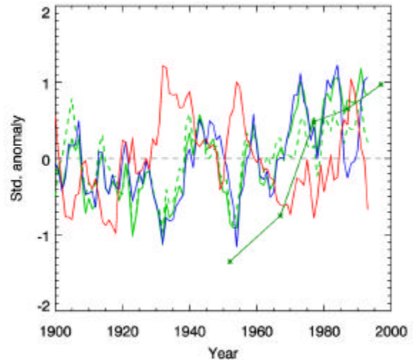
Figure 1: Long-term variations (1900-1993) in annual averages of conterminous U.S. climate (air temperature (red), precipitation (blue)) and simulated carbon cycle variables (net primary production, solid green and net ecosystem production, dashed green) smoothed with a 5 point binomial filter. Ground based estimates of net primary production (green with symbols) are derived from national forest assessments reported between 1952 and 1997.
