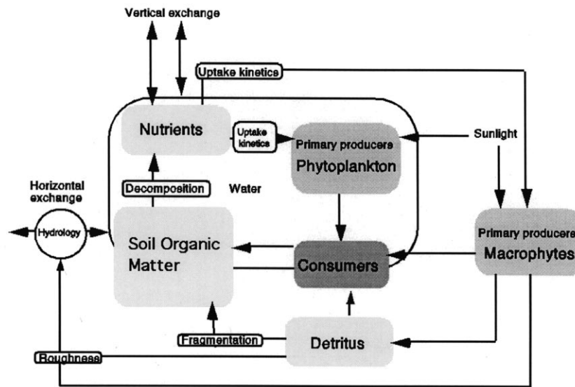
Fig. 3. Material flows between ecosystem components as modeled within a Pat_GEM unit.
