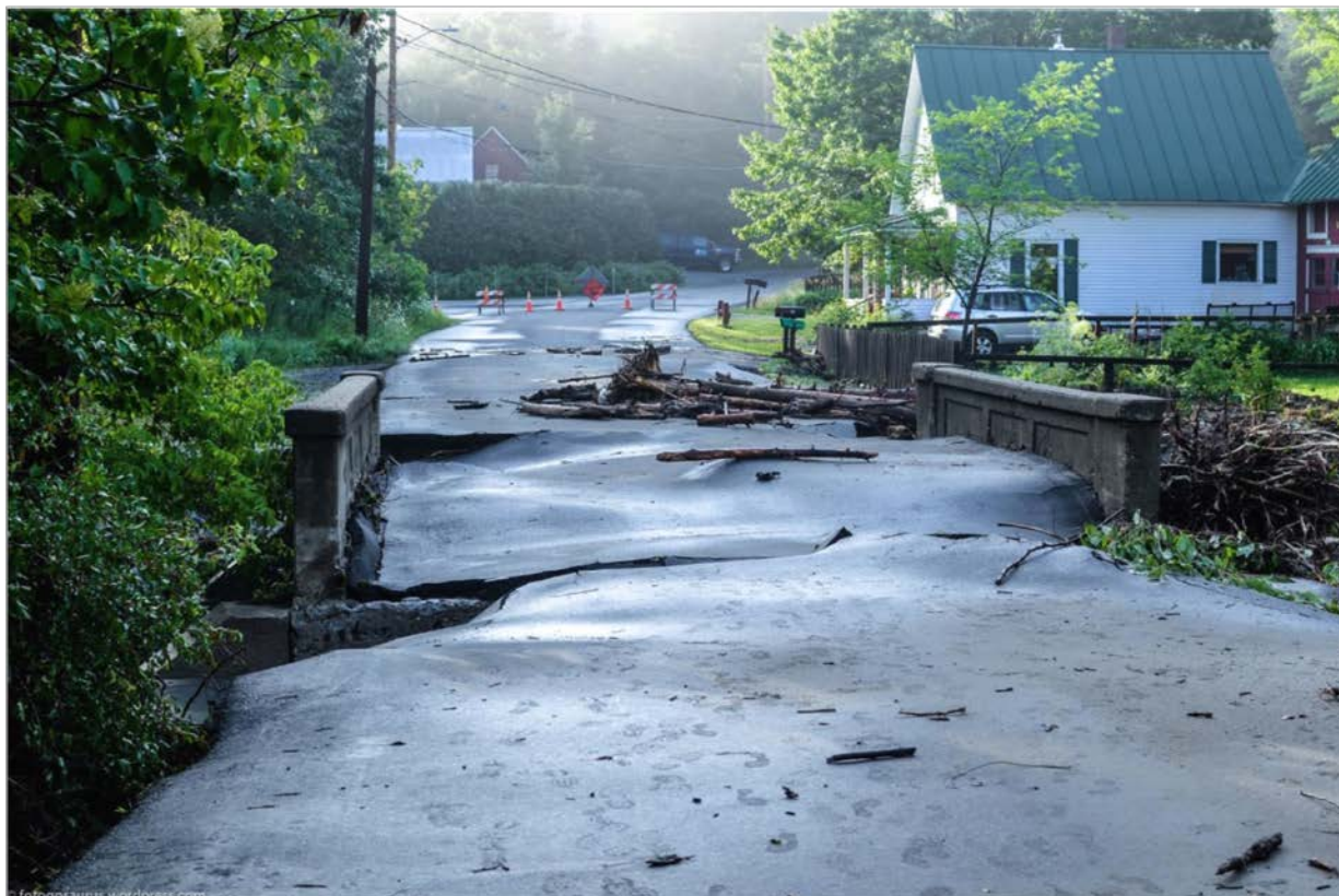
Figure 1 Damage caused by debris blockage of a crossing structure
