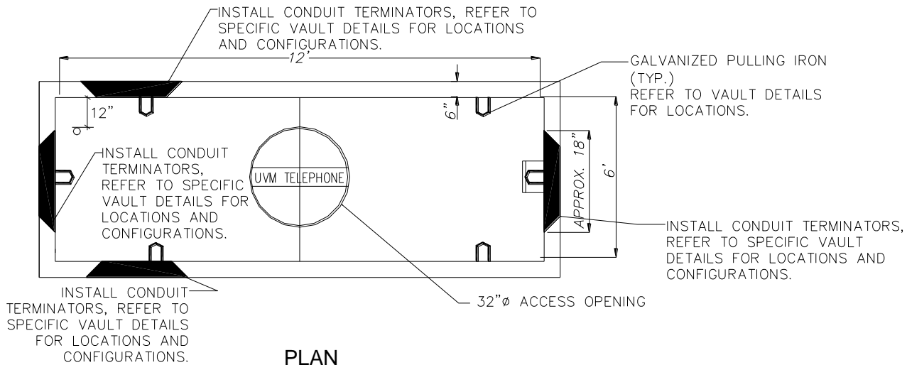
Detail #1 Typical Precast Vault Detail
