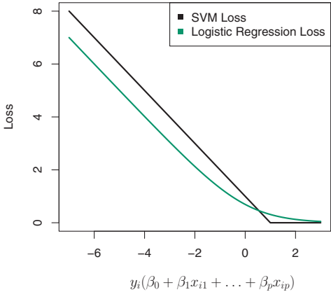
FIGURE 9.12. The SVM and logistic regression loss functions are compared, as a function of y_i(\beta_0 + \beta_1x_{i1} + \dots + \beta_px_{ip}) . When y_i(\beta_0 + \beta_1x_{i1} + \dots + \beta_px_{ip}) is greater than 1, then the SVM loss is zero, since this corresponds to an observation that is on the correct side of the margin. Overall, the two loss functions have quite similar behavior.
