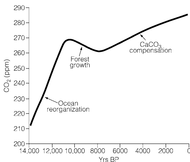
Figure 3. Proposed explanation of late-Holocene \text{CO}_2 rise based on ocean carbonate compensation (Broecker et al., 1999).
