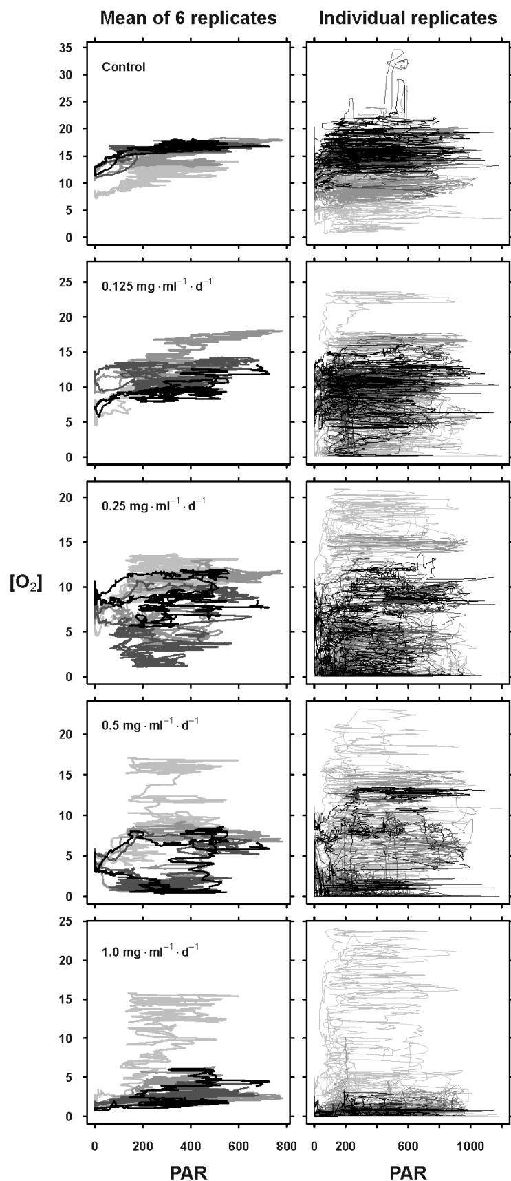
Figure S14 – Plots of [O_2] as a function of PAR for each prey-addition treatment (top to bottom: controls to 1.0 \text{ mg} \cdot \text{ml}^{-1} \cdot \text{d}^{-1} ). Gray-scale indicates the four days of prey additions, from day 1 (light gray) through day 4 (black). Plots in the left column are the means of all six replicates in each treatment, whereas plots in the right column shows time-series traces of all six individual replicates.
