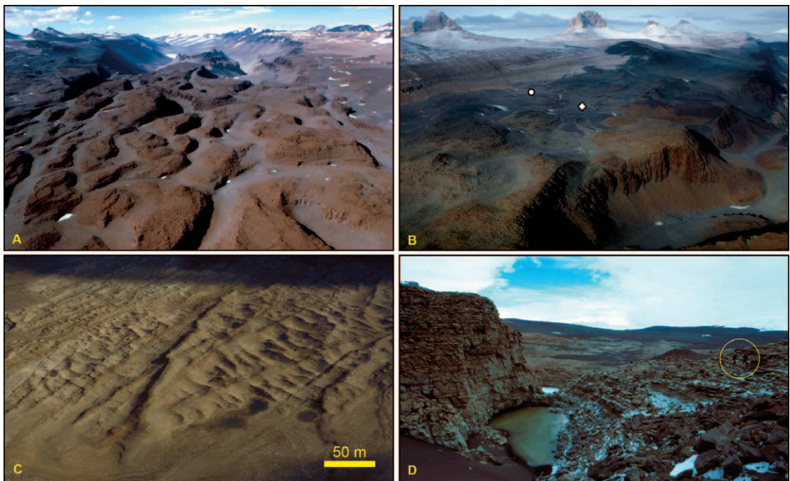
Figure 2. A: Oblique-aerial view of channels incised into lower surface (ES3) of Labyrinth; channels in foreground are ~100 m wide; main trough of Wright Valley is in background. B: Oblique-aerial view of ES1 and ES2 with deep crosscutting channel of ES3 in foreground. Irregular dark patches on ES1 and ES2 are scattered deposits of stratified sand and gravel; circle and diamond (1.2 km apart) show locations of in situ (ALS-00–102) and reworked ash (ALS-00–145B), respectively. C: Low-elevation aerial view of scoured-bedrock terrain in central Wright Valley; \lambda = \sim 22 m, with amplitudes of ~2–4 m (see text); mafic dikes cut obliquely across this corrugated, granitic bedrock. D: Oblique-aerial view of a 50-m-wide pothole incised into sandstone bedrock, Convoy Range; scoured bedrock terrain is in background. Geologists are circled for scale.
