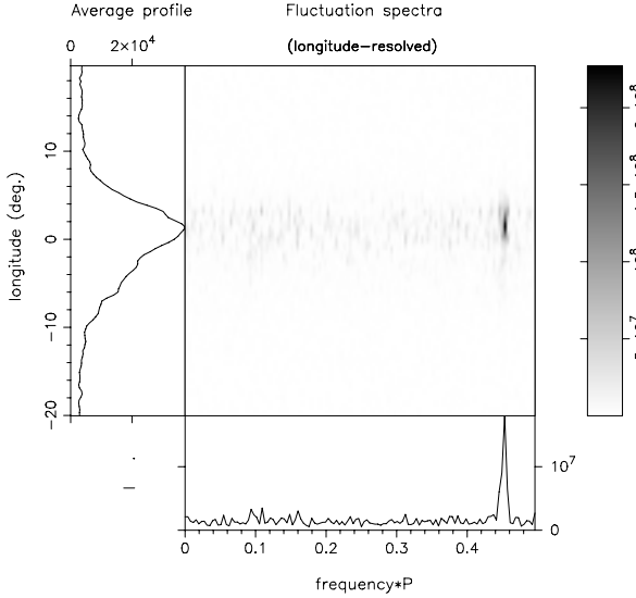
Fig. 7. Longitude-resolved fluctuation spectra computed from 256 pulses just after the B-mode onset of the 2003 March 10 observation. Here the “drift” feature frequency is 0.452 c/P_1 , which corresponds to a 20-subbeam “carousel” circulation time of 36.47 \pm 0.03 P_1 – just the same as that determined for the Q-mode in Fig. 6.
