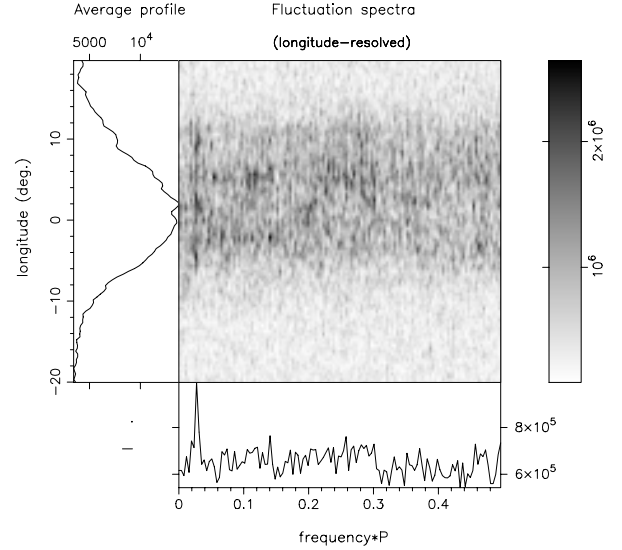
Fig. 6. Longitude-resolved fluctuation spectra for the initial Q-mode interval of the 2003 March 10 observation. The prominent feature in the bottom panel at 0.0275 \pm 0.001 \cdot c/P_1 corresponds to an interval of 36.4 \pm 0.9 \cdot P_1 – apparently the first detection of a Q-mode circulation time. Note also the complete lack of a B-mode "drift" feature at about 0.45 \cdot c/P_1 and the broad, single Q-mode profile centered at zero longitude. These MJD 52709 spectra were computed using the first 2048 pulses, whereas the B-mode recommences at about pulse 2540.
