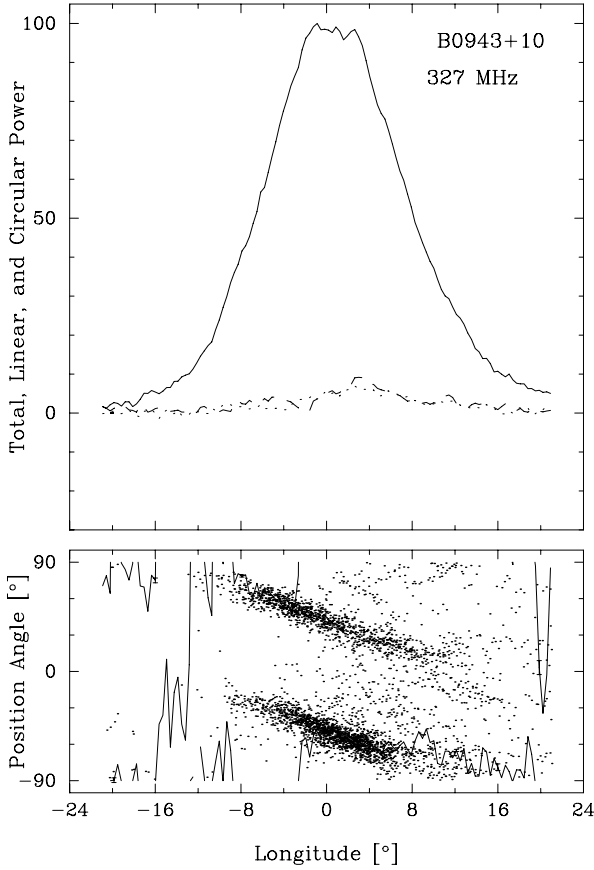
Fig. 2. Average polarization profile and polarization-angle distribution as in Fig. 1 for the Q-mode of PSR B0943+10. This 327-MHz observation was recorded on 2003 October 4.
