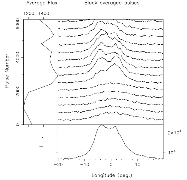
Fig. 3. A set of total intensity pulse profiles of B0943+10 at 327 MHz (2003 March 10), obtained by integration of 482 consecutive pulses. The first 5 integrations show the smooth, broad and weak profiles of the Q-mode. Note the unusual profile shape just after the burst-like B-mode onset with the strongest emission coming after the magnetic-axis (zero) longitude. The subsequent profiles show the gradually decreasing intensity of the second component. The broad shape of the total integration in the bottom panel shows that Q-like features persist well after the B-mode onset. The intensity integrated over the pulse window as a function of pulse number is shown in the left-hand panel.
