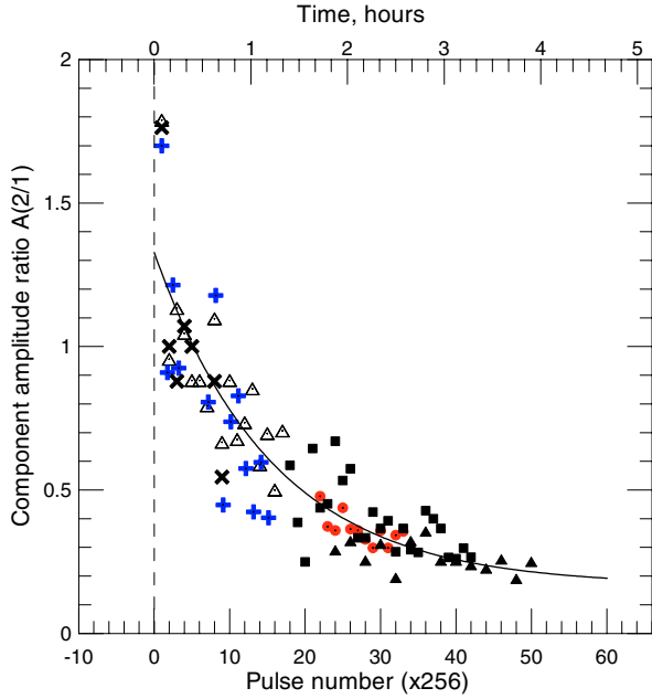
Fig. 5. Systematic changes in B0943+10's average-profile form as a function of time after the B-mode onset. Initially the trailing component dominates, but its profile slowly evolves to its usual asymptotic form, where the longitude of the magnetic axis falls near the trailing half-power point and the intensity of the second component decreases to 1/5 that of the first, dominant component. Here, we plot the amplitude ratio A(2/1) of the two component peaks, separated by 6^\circ longitude, as a function of time in terms of the profile number. Each average is comprised of 256 individual pulses, or 280 s (4.7 min). Note the remarkable similarity of the very first B-mode pulse shape with A(2/1) near 1.75 for all three Q- to B-mode transition days (hereafter MJD 52709 open triangles, 52832 Xs, 52916 crosses). Values for the "pure B" days (MJD 52711 squares, 52840 triangles and 52917 circles) are shifted to begin at profile numbers 18, 24 and 22, respectively. They clearly show a gradual change of pulse shape and seem to represent a later portion of the Q- to B transformation process (see also Fig. 10). This interpretation is further supported by the gradually increasing circulation time of all three "pure B" days (see text and Fig. 8). The vertical dotted line indicates the B-mode onset time. A fit to the values (solid curve) has the form 0.17 + 1.16 \exp(-t/\tau) , where \tau is 15.65 \cdot 256 \cdot P_1 blocks.
