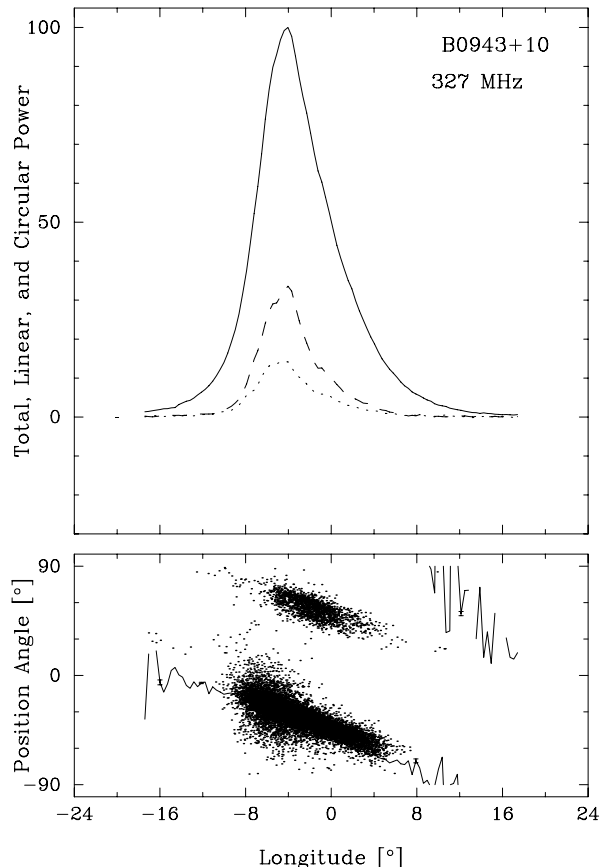
Fig. 1. Average polarization profile giving the total intensity (solid line), total linear (dashed line) and circular polarization (dotted line) for the B-mode of PSR B0943+10 ( top panel ). Linear polarization angles for the integrated profile (solid line) and sufficiently strong individual pulse samples (dots) are given as a function of pulse longitude ( bottom panel ). The 327-MHz PS was recorded on 2003 October 5.
