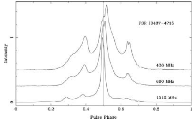
Figure 8. Total-intensity profiles for J0437–4715 at 438, 660 and 1512 MHz, which have been aligned according to the zero-crossing point of the antisymmetric circular polarization under their central components from (Navarro et al. 1997, their fig. 5). Note that the notches almost align – and that they could even do so more closely if only a slightly different alignment had been used.
