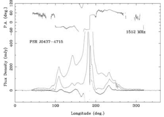
Figure 7. Polarized pulse profile for J0437–4715 at 1512 MHz from (Navarro et al. 1997, their fig. 4).
