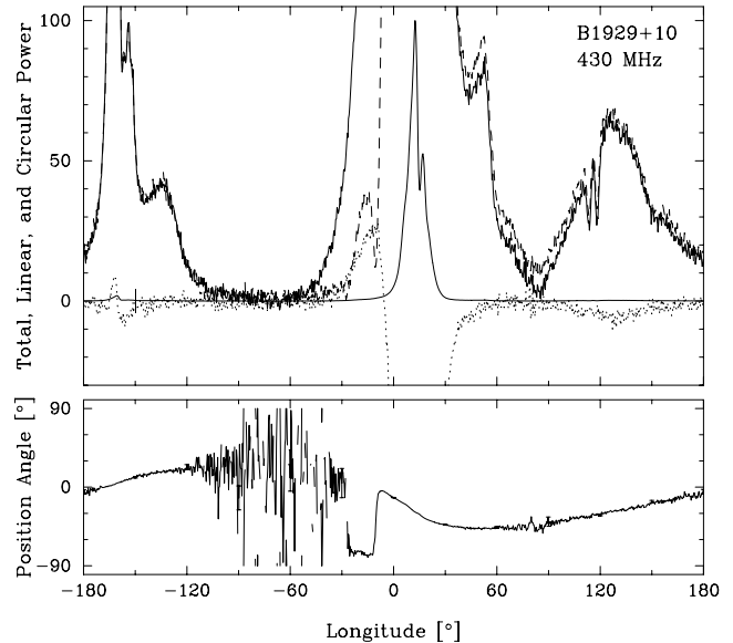
Figure 5. Full-period average polarization profile of B1929+10 at 430 MHz, after Rankin & Rathnasree (1997). The total power (Stokes I ) is plotted first at full scale and then at a \times 250 expanded scale, so that only features below 0.4 per cent of the MP amplitude are now visible. The linear ( L ) and circular ( V ) polarization are then plotted at the expanded scale. The PA is plotted in the lower panel. Note the double notch feature that follows the MP by about 100^\circ . This region exhibits complete linear polarization (see text), so the notches are clearly visible in both I and L , representing an intensity decrease at their centres of some 40 per cent.
