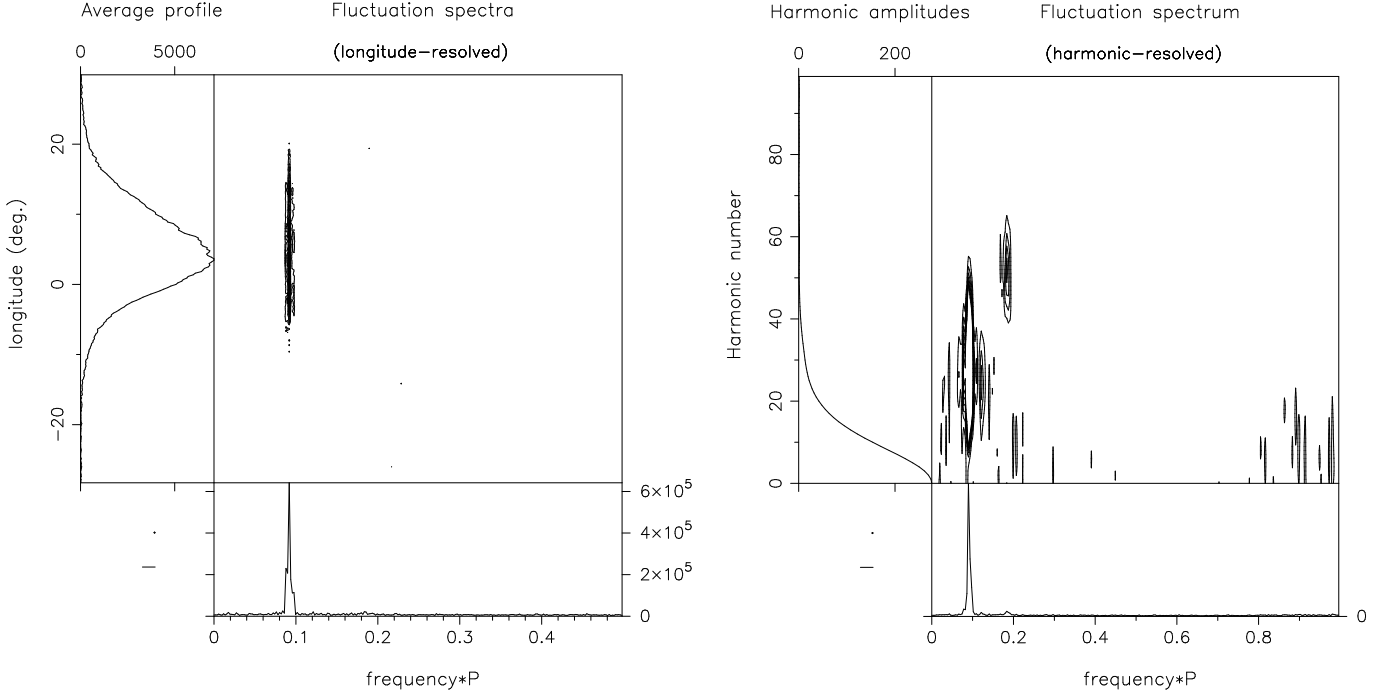
Fig. 1. Longitude-resolved ( a , left) and harmonic-resolved ( b , right) fluctuation spectra for pulsar B0809+74 at 328 MHz, computed using a WSRT PS recorded on 2000 November 26. The analysis was applied to the total power (Stokes I ) and used FFTs of length 512 and 256, respectively. The three panels of the left-hand LRF display give the pulsar’s average profile (left), LRF spectra (centre), and integral spectrum, (bottom) respectively; whereas, those of the right-hand HRF display give the (integer) harmonic amplitudes of the average profile (left), the non-integer harmonic amplitudes associated with the modulation (centre), and the integral fluctuation spectrum (bottom). See DR01 for a complete description. The central panels of both displays use 8 contour levels; however, these cover only the lowest 5% of the feature amplitude of the HRF spectrum in order to exhibit the lowest level features. Note also that the longitude origin of the average profiles has been taken just above the half-power point on the profile’s leading edge, following the analysis of Paper I.
