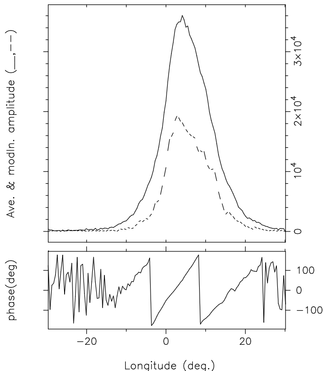
Fig. 2. Fluctuation-spectral phase and modulation amplitude at 328 MHz corresponding to the primary 0.092\ c/P_1 feature in Fig. 1a and b. Fluctuation power is plotted as a function of longitude within the average profile in the top panel, whereas the fluctuation phase is given in the lower panel.
