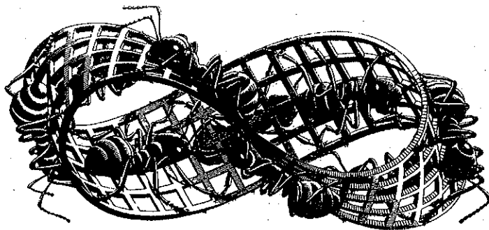
FIGURE 1.3: Möbius Strip II, by M. C. Escher. (© Cordon Art; reprinted with permission)
