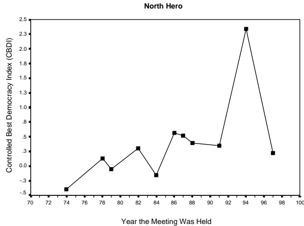
Plot 3 Controlled Best Democracy Index (CBDI) 1974-1997
