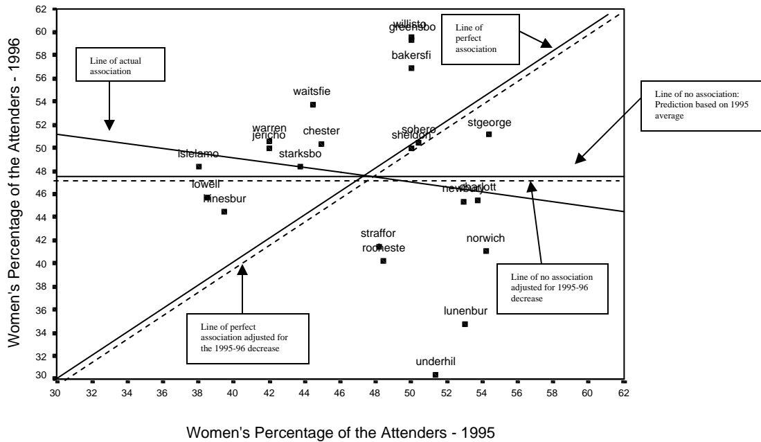
Plot 2 The Weakest Association: R2 = .02
