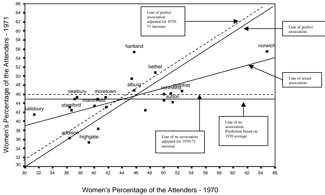
Plot 2 The Weakest Association: R2 = .02
