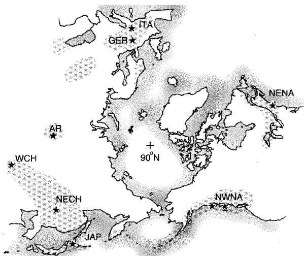
FIG. 1. Geographical distribution of Polystichum braunii accessions, north-polar view. Range of P. braunii indicated by tiled fern motif. AR = Altai, Russia. GER = Germany. ITA = Italy. JAP = Japan. NECH = northeastern China. NENA = northeastern North America. NWNA = northwestern North America. WCH = western China.
