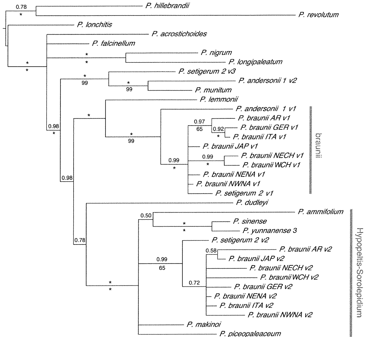
FIG. 5. Phylogram based on combined gapCp and pgiC data. Variants are distinguished with v# suffixes to the accession names. Bayesian posterior probabilities (above branches) and maximum parsimony bootstrap percentages (below branches) given where support values exceed 0.5 or 50% respectively. Asterisk indicates 1.0 PP or 100% BS. AR = Altai, Russia. GER = Germany. ITA = Italy. JAP = Japan. NECH = northeastern China. NENA = northeastern North America. NWNA = northwestern North America. WCH = western China.
