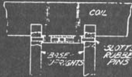
METHOD OF ANCHORING COIL TO BASE
