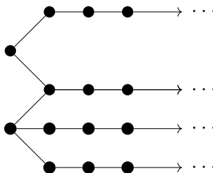
Figure 8.3: [GN95] computes \Gamma_0(xy) \setminus \mathcal{I} “layer by layer”
