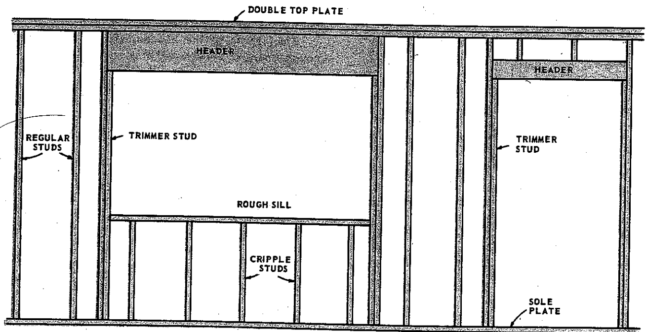
Fig. 8-8. Framed openings in platform construction. Note the header size is larger than required, but fills the space completely thus saving labor in cutting and assembling cripples.
