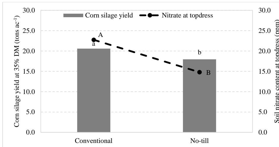
Figure 6. Corn silage yield and soil nitrate content at topdress by tillage treatment.
