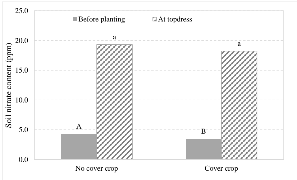
Figure 3. Soil nitrate content before planting and at the time of topdress. Treatments with the same letter performed statistically similarly to one another.
