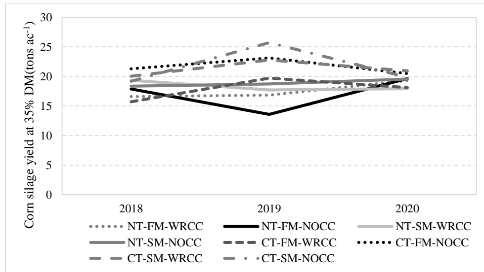
Figure 1. Treatment x year interaction for corn silage yield.
