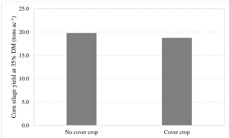
Figure 4. Corn silage yield by cover crop treatment. Cover crop treatments performed statistically similarly to one another.
