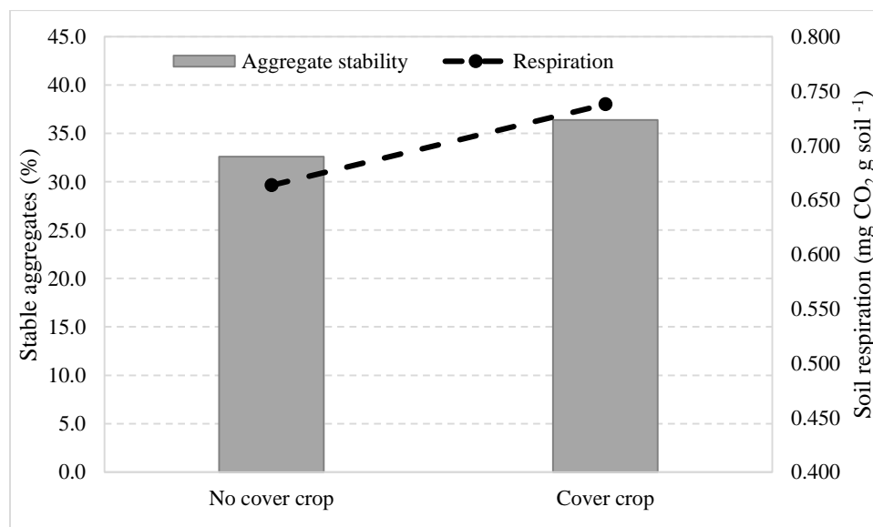
Figure 2. Soil aggregate stability and respiration by cover crop treatment.
