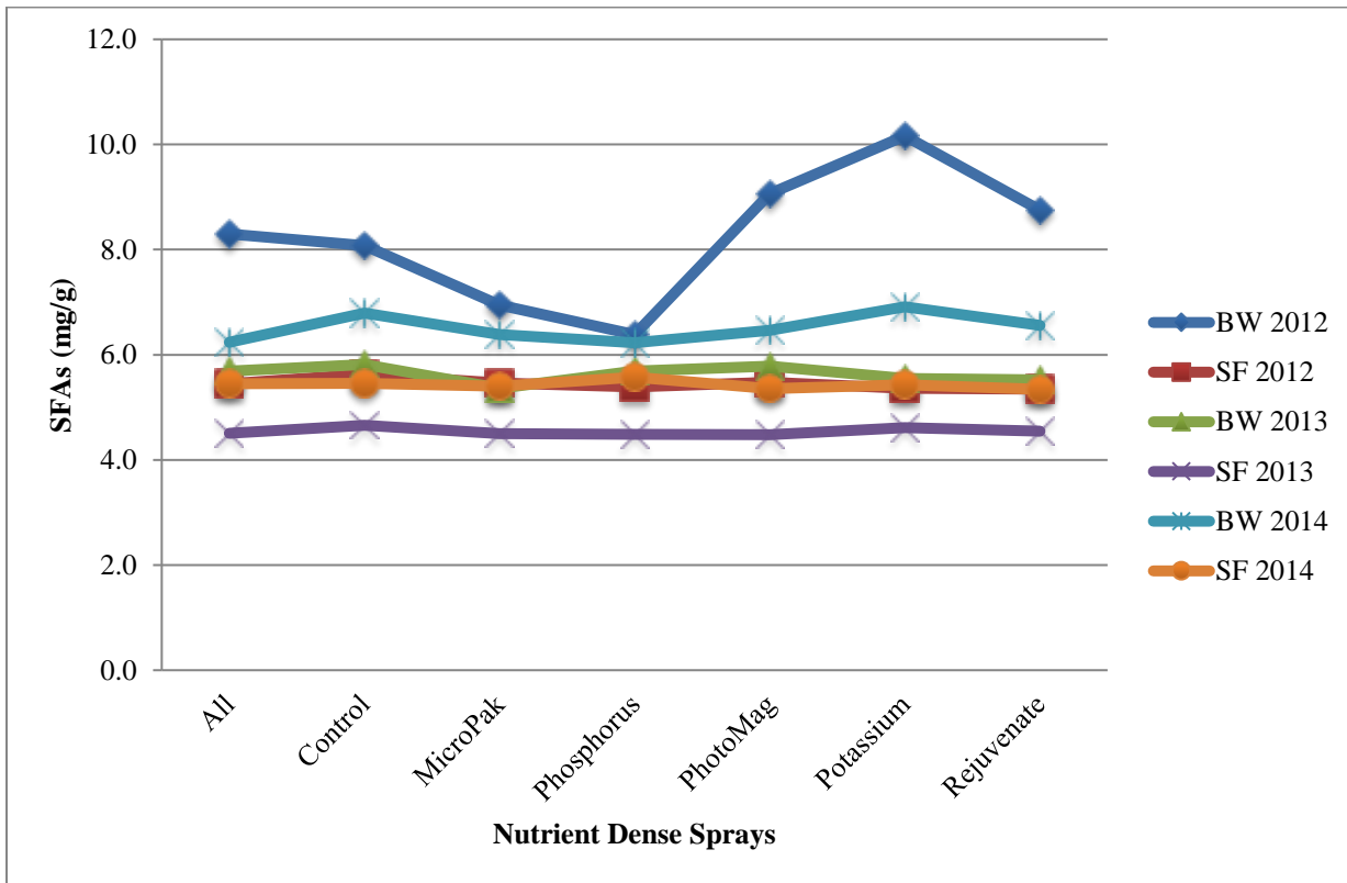
Figure 2. Concentration of SFAs by site-year and Nutrient Dense Spray treatment.
