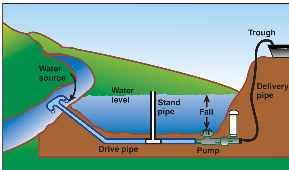
Typical ram pump set-up.
