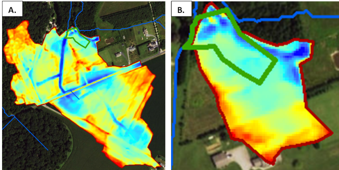
Figure 18. Topographic Openness for CP22 in Choptank watershed: potential contributing area (A.) of approximately 72 acres (29 ha) intersected by ditches that limit the buffer effective contributing area (B.) to 5 acres (2 ha), only 15% of the potential contributing area.
