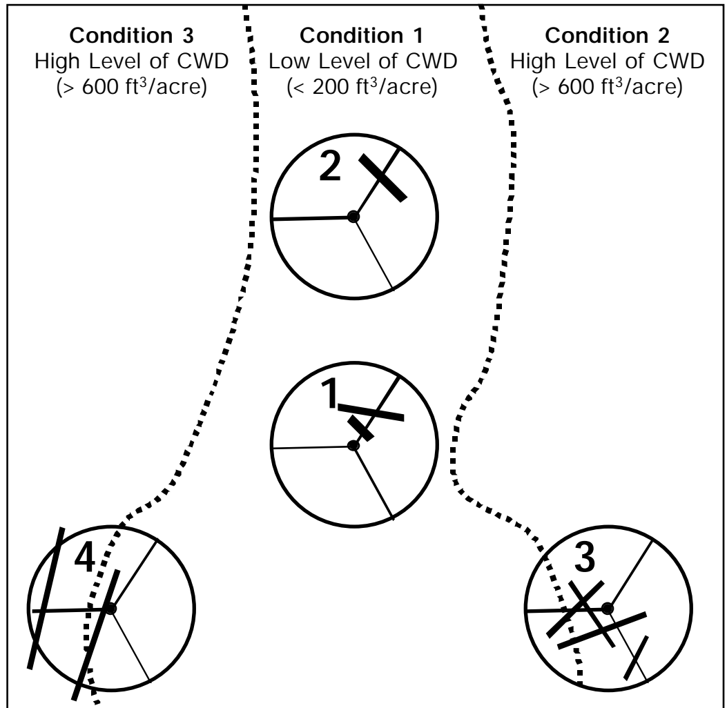
Figure 8.1.—Hypothetical plot map and corresponding condition classes for CWD estimation procedure example one, appendix 8.1.
