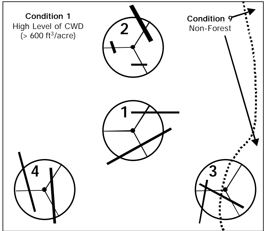
Figure 8.2.—Hypothetical plot map and corresponding condition classes for CWD estimation procedure example two, appendix 8.2.
