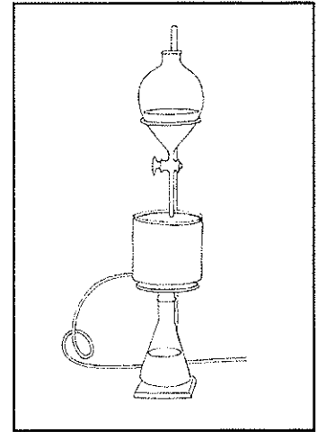
Fig. 14. Apparatus for extracting thrips from soil.
