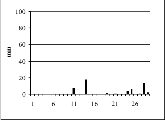
CASTNet: April
