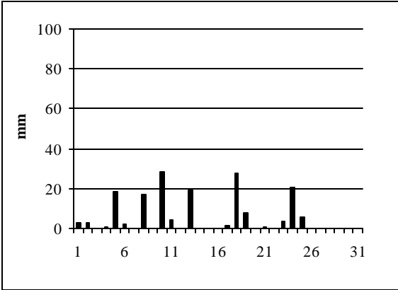
CASTNet: May
