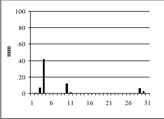
CASTNet: March
