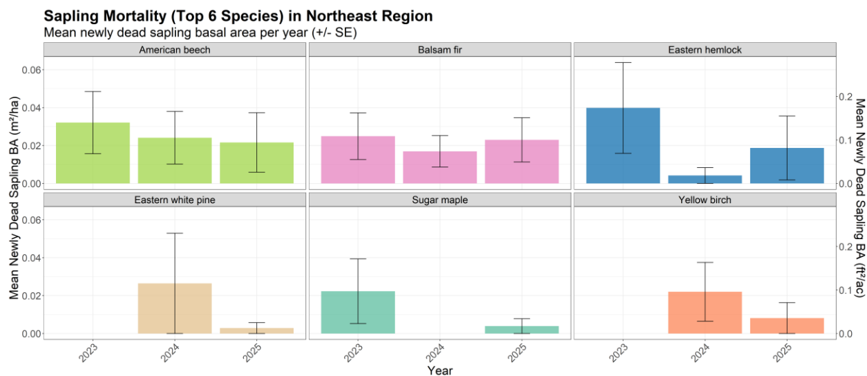
Figure 26. The top six species experiencing the greatest sapling mortality across the Northeast region, shown as basal area per hectare ( \text{m}^2/\text{ha} , left axis) and acre ( \text{ft}^2/\text{ac} , right axis) lost per year. Only species with more than ten individuals in the sample were assessed for inclusion in this chart.
