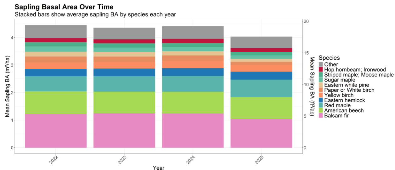
Figure 28. Overall sapling basal area composition in hectares ( \text{m}^2/\text{ha} , left axis) and acres ( \text{ft}^2/\text{ac} , right axis) throughout the Northeast region for all species each year. The ten species with highest basal area are shown individually, while all other species are grouped as “Other.” The overall bar height indicates total sapling basal area per hectare and acre regionally for each year.
