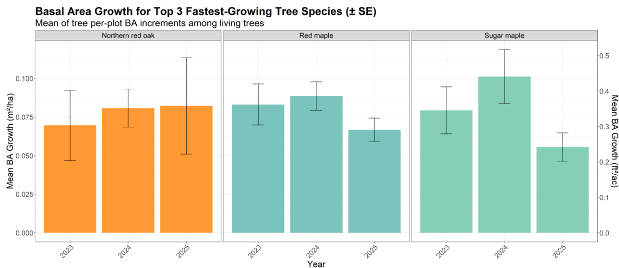
Figure 17. The top three species with the greatest average basal area growth across the Northeast region. Bars represent the mean basal area increment in hectares ( m^2/ha , left axis) and acres ( ft^2/ac , right axis) each year. Error bars represent the standard error of individual growth in basal area within each species.
