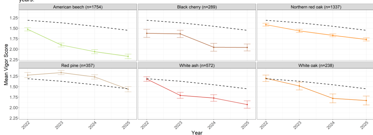
Figure 12. Top six tree species with the greatest decline in vigor (highest stress levels) over time across the Northeast region, among species comprising at least 0.5% of total basal area region wide. Vigor scores range from 4 (severe decline) to 1 (healthy), with intermediate values for trees in decline. The dashed black line provides an overall trend for comparison across all species, and the error bars show the standard error of the vigor score per species and year. Note that the y-axis is inverted to aid interpretation, because
