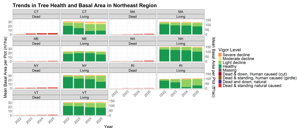
Figure 10. Region-wide mean basal area per plot in hectares ( \text{m}^2/\text{ha} , left axis) and acres ( \text{ft}^2/\text{ac} , right axis) for living and dead trees across different tree vigor classes. Data are grouped by tree status, with living classes shown on the right and dead classes on the left.
