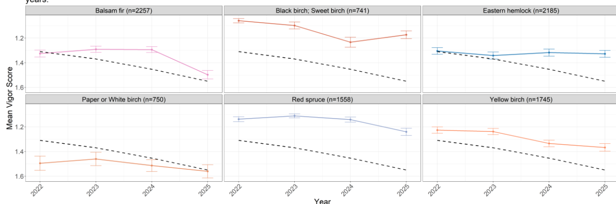
Figure 11. Top six tree species with the healthiest vigor (lowest stress levels) over time across the Northeast region among species comprising at least 0.5% of basal area regionally. Vigor scores range from 4 (severe decline) to 1 (healthy), with intermediate values for trees in decline. The dashed black line indicates the overall region-wide vigor trend across all species. Error bars represent the standard error of the vigor score for each species and year. Note that the y-axis is inverted to aid interpretation, because higher vigor scores indicate worsening tree condition while lower scores represent healthier trees.
