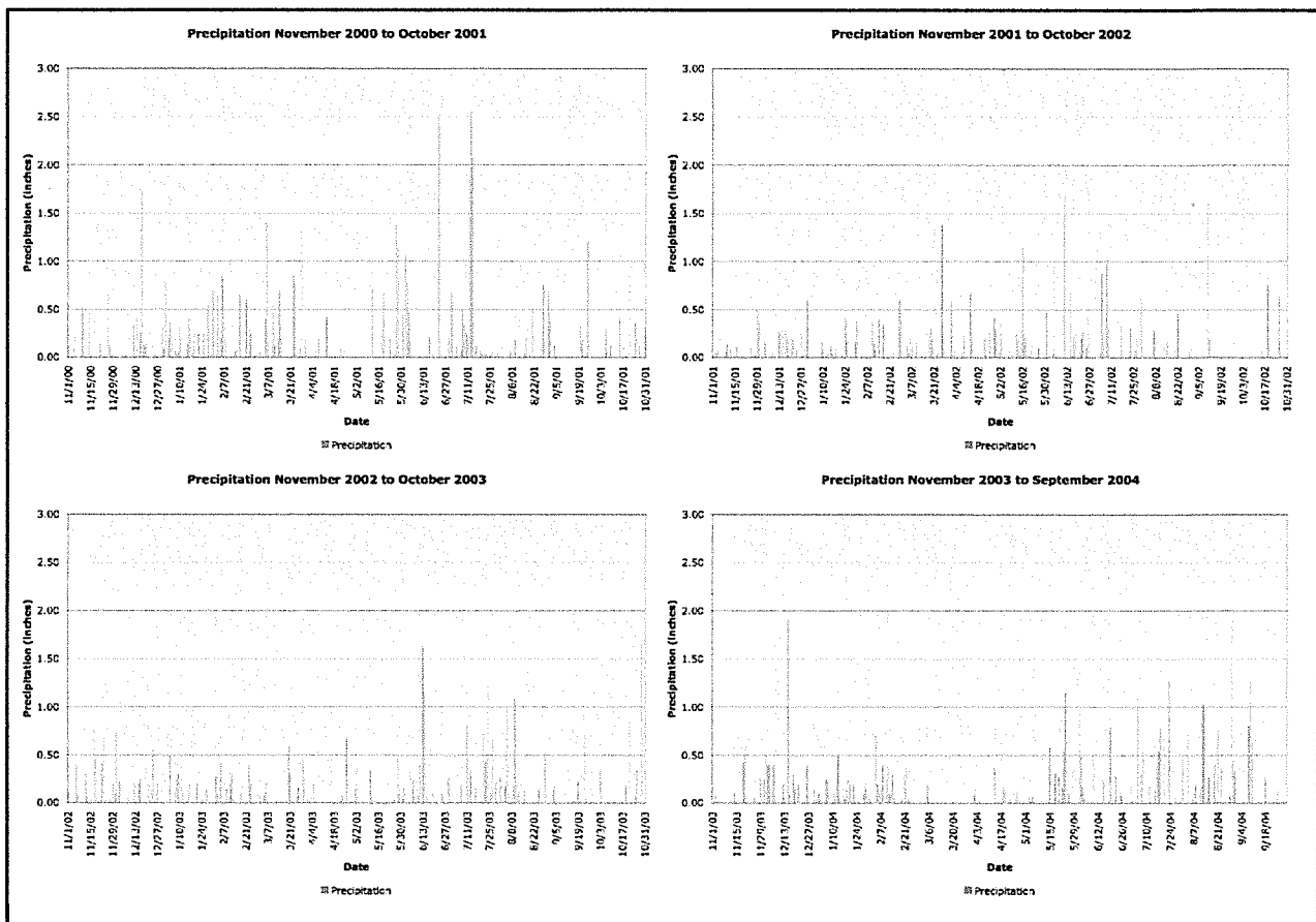
Figure 8. Precipitation
