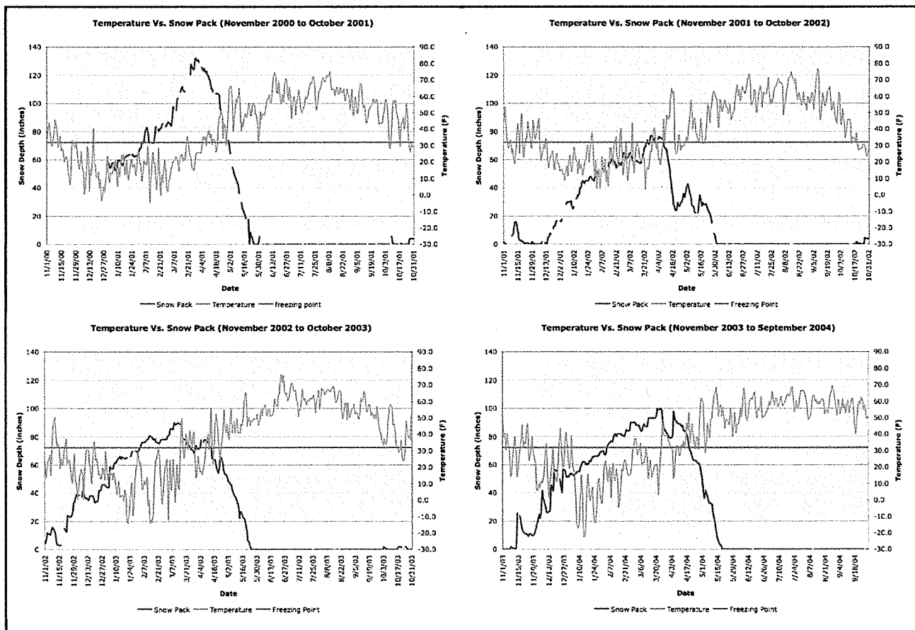
Figure 13. Temperature Vs. Snow Pack
