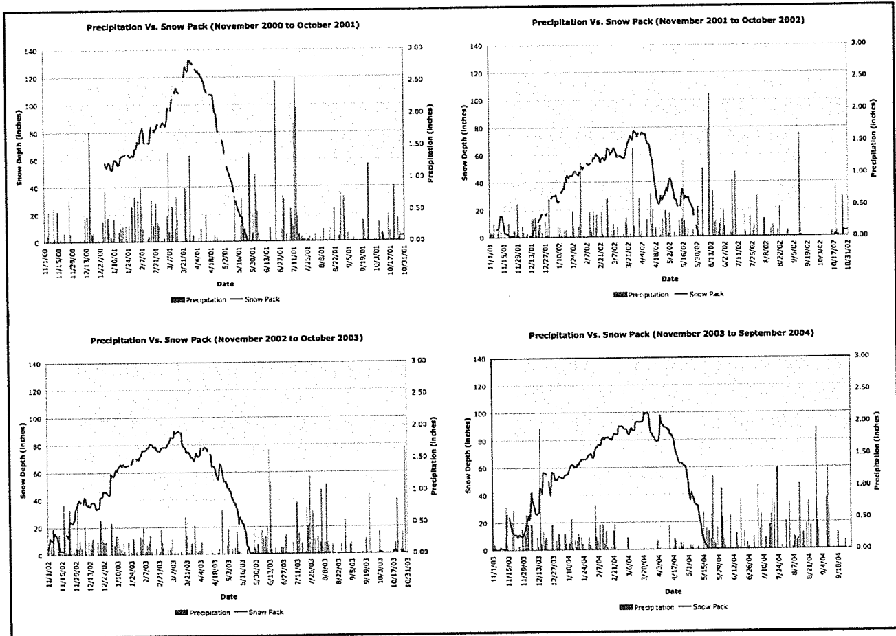
Figure 12. Precipitation Vs. Snow Pack
