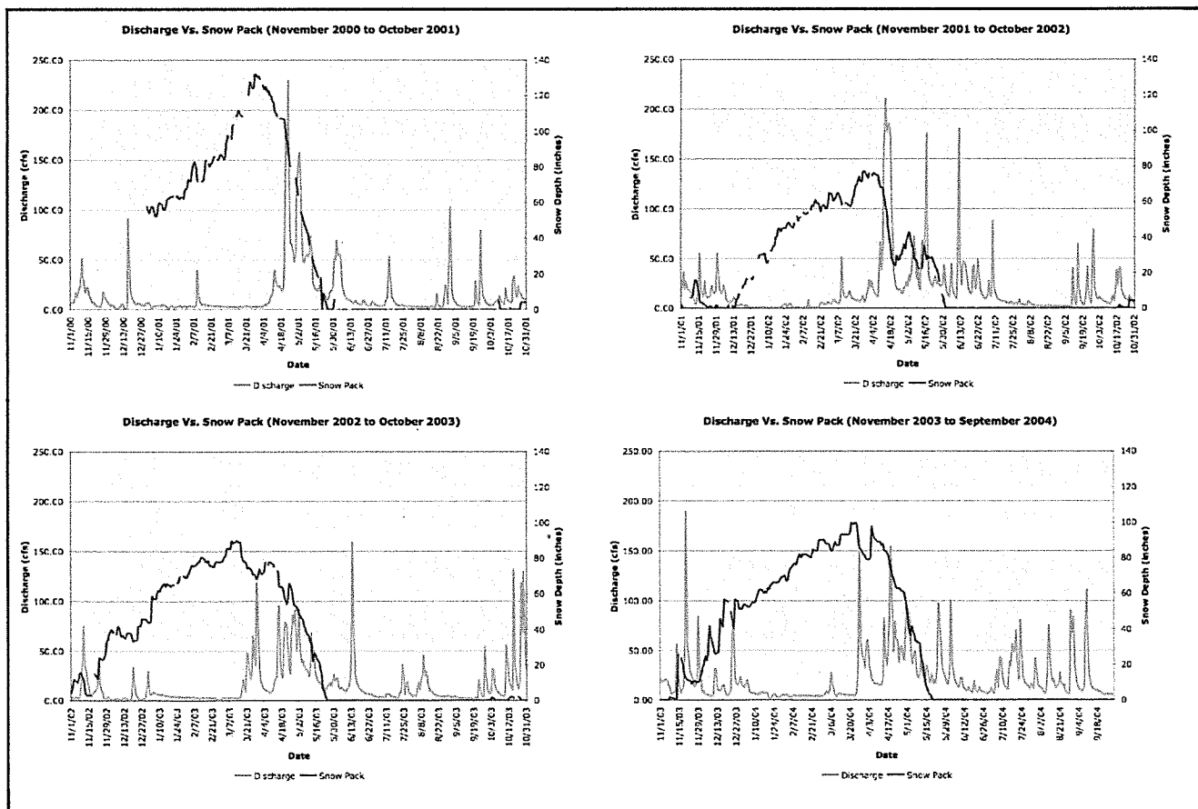
Figure 14. Discharge Vs. Snow Pack
