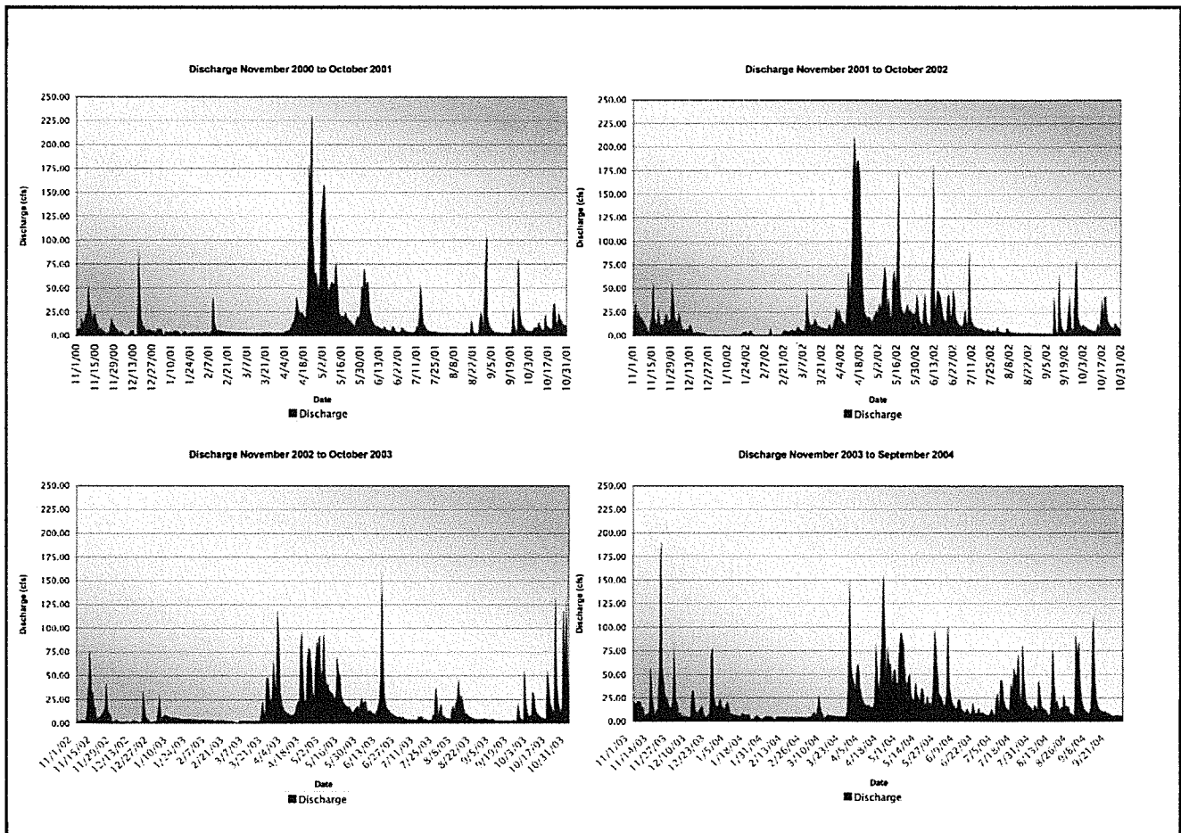
Figure 7. Discharge
