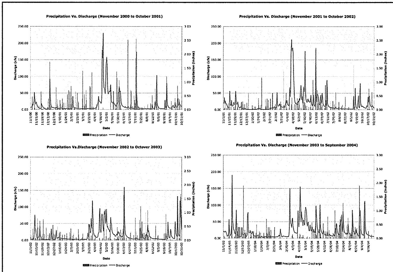
Figure 11. Precipitation Vs. Discharge
