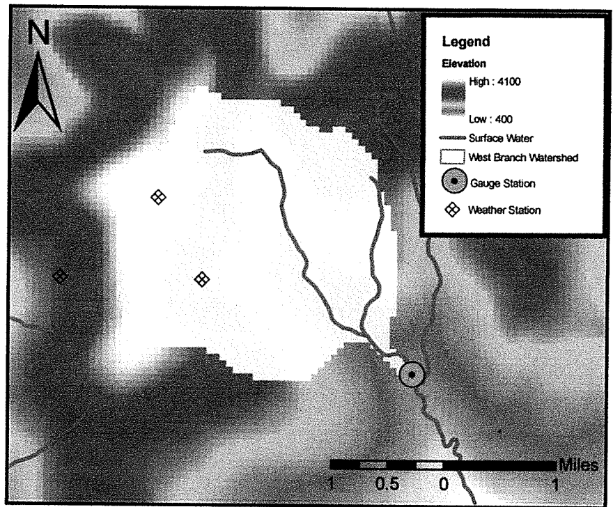
Figure 4. GIS Generated Watershed Delineation
