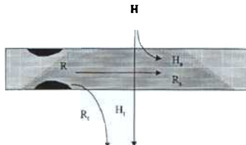
Figure 3. Components of the sediment budget constructed at the scale of individual road segments. Inputs include sediment mobilized from hillslopes or in stream channels above roads ( H ) and sediment mobilized from within the road prism ( R ). Sediment contributed to or mobilized on the road could be stored ( H_s , R_s ) or transported downslope ( H_t , R_t ).
