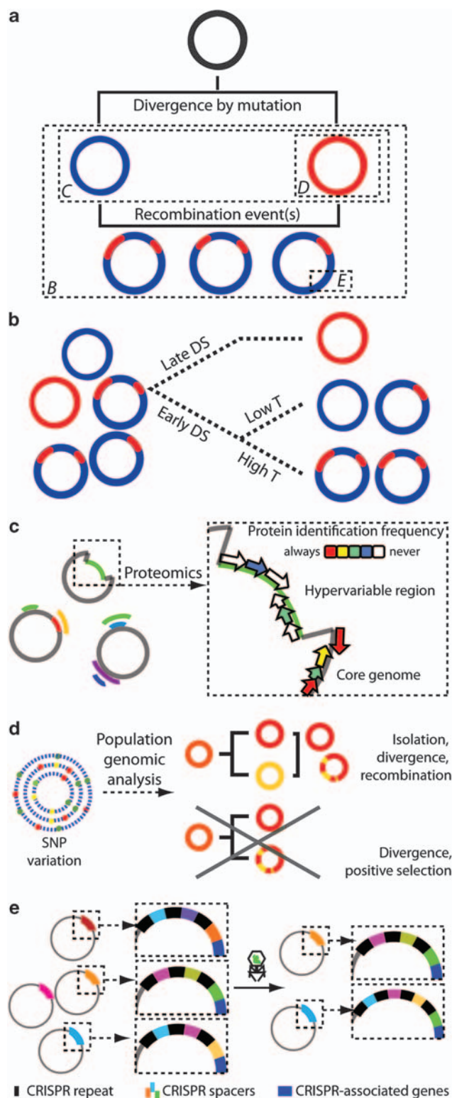
Figure 3 Insights into links between evolutionary and ecological processes at different levels of resolution. (a) Although insights were derived for many archaeal and bacterial populations, this figure just focuses on the dominant Leptospirillum Group II bacteria. Two populations that derived from a common ancestor, as well as variants arising from recombination between them, are found in the Richmond Mine. Rectangles group the population(s) for which more details are shown in b–e. (b) The ecological distribution of the two populations and their recombinants primarily correlates with biofilm developmental stage (DS) and temperature (T). (c) Proteins encoded in hypervariable regions were rarely identified by proteomics, indicating that many have little or no role in environmental adaptation. Differential expression of shared genes is implicated in ecological divergence. (d) Population genomic analysis of single-nucleotide polymorphisms (SNPs) indicated variation within one population is not maintained by positive selection, but rather reflects allopatric divergence, migration and recombination, with some loss of variants. (e) Variation approaching the individual level is apparent in the clustered regularly interspaced short palindromic repeat (CRISPR) loci, which provide immunity against predation by specific viral/phage variants. Patterns of variation indicate that viral predation can shape population and community structure. Similar ‘hot spots’ of variability are found elsewhere in the genome, for example, at loci encoding cytochromes involved in Fe oxidation, raising questions about their potential role in fine-scale environmental adaptation.
