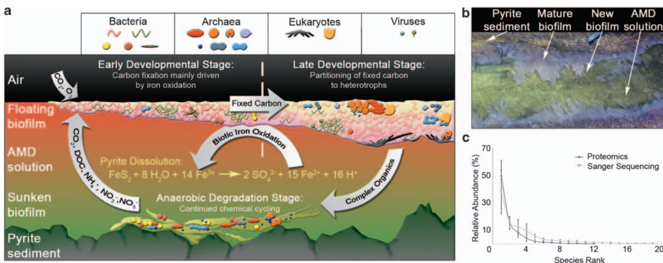
Figure 1 (a) Schematic illustrating important features that make the AMD system a good model for studying microbial communities (for example, relatively low species complexity, defined ecological succession patterns and trophic levels, tight biological–geochemical coupling, high biological productivity). (b) Picture of in situ biofilm developmental stages. (c) Rank–relative abundance curve for the AMD system communities. Sequencing reads from three Sanger sequencing libraries (~100 Mb each) that overlapped with a 16S rRNA gene were identified based on the best match in a database specific for the AMD system using BLAST. Proteomics data were analyzed by assigning each identified protein to the corresponding organism and calculating its relative representation as a fraction of all proteins identified. Error bars indicate the s.d. for each rank across samples. Although diversity is lower in the AMD system, the relationship is similar to various more complex systems (see for example Fuhrman et al. , 2008).
