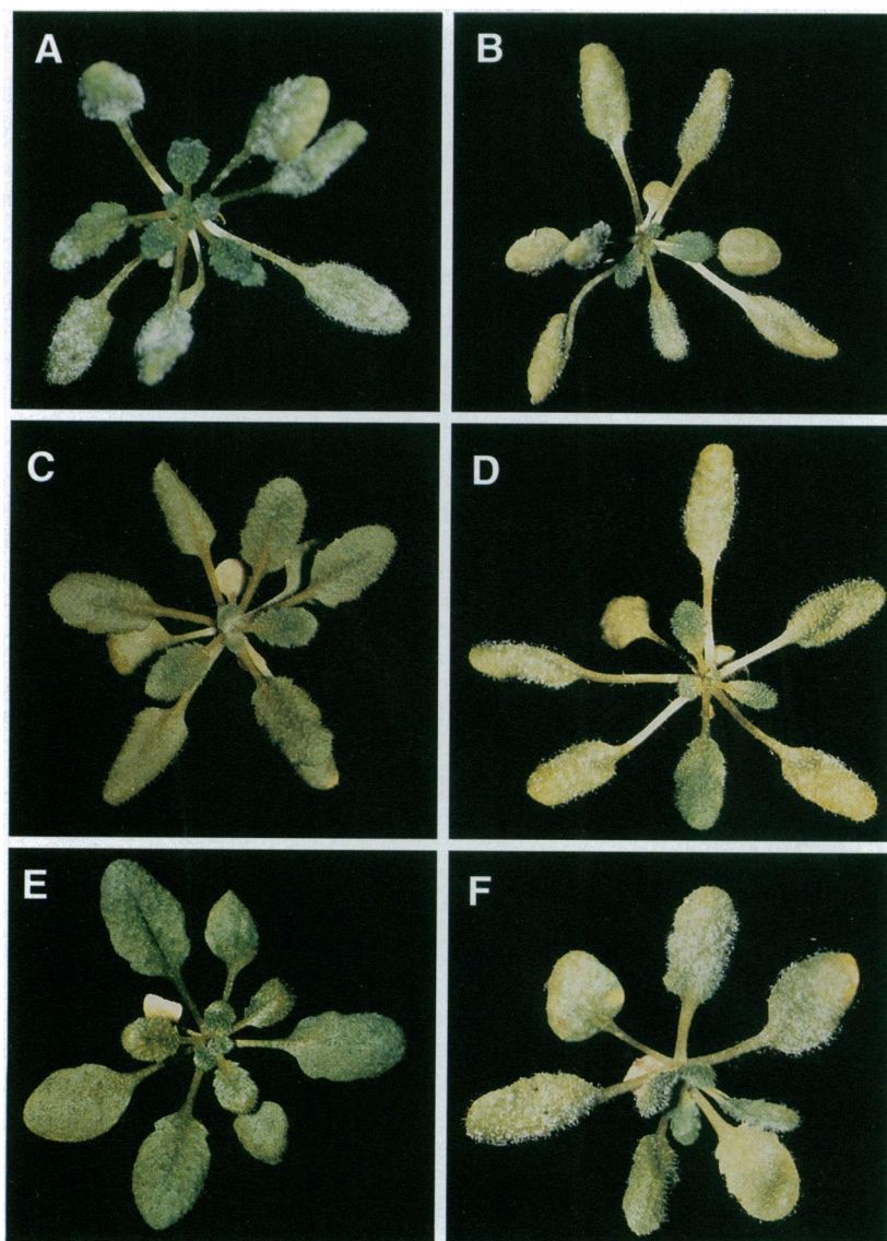
FIG. 1. nim1 plants are defective in acquired resistance to P. parasitica following treatment with SA or INA. Wild-type ( A , C , and E ) and nim1 ( B , D , and F ) plants were treated with water ( A and B ), INA ( C and D ), or SA ( E and F ). Four days later, plants were inoculated with a P. parasitica pv. Emwa conidial suspension. Evaluations and photographs were made 7 days later. After each treatment, fungal growth on nim1 was indistinguishable from that on water-treated wild-type plants.
