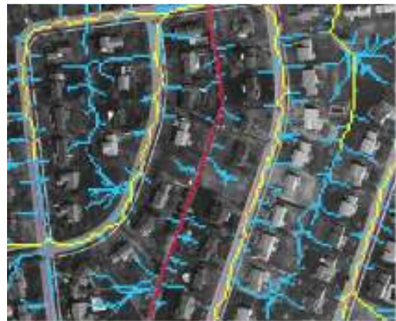
Figure 8. Micro Stormwater Drainage Network calculated using LiDAR data.
