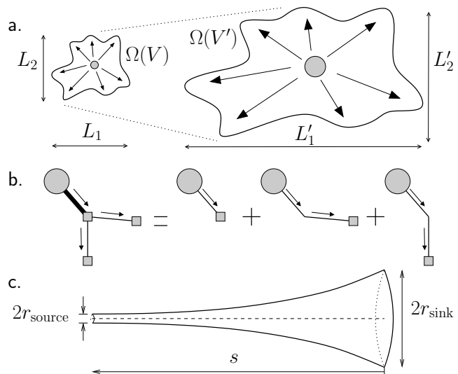
FIG. 1: (a) We consider families of d -dimensional spatial regions that scale allometrically with L_i \propto V^{\gamma_i} , and exist in a D -dimensional space where D \geq d . For the d=D=2 example shown, \gamma_{\max} = \gamma_1 > \gamma_2 , and L_1 grows faster than L_2 . We require that each spatial region is star-convex, i.e., from at least one point all other points are directly observable, and the single source must be located at any one of these central points. (b) Distribution (or collection) networks can be thought of as a superposition of virtual vessels. In the example shown, the source (circle) supplies material to the three sinks (squares). (c) Allowing virtual vessels to expand as they move away from the source captures a potential decrease in speed in material flow. For scaling of branching network form to be affected, the radius r of a virtual vessel must scale with vessel length s (measured from the sink) as s^{-\epsilon} .
