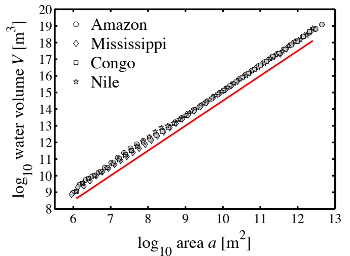
FIG. 2: The scaling of network volume versus basin area for four continental-scale river networks. The solid line indicates a scaling of 3/2 . Network volume is estimated for an idealized steady-state, uniform rainfall condition normalized such that V_{\text{net}} = \sum_{ij} a_{ij} , where a_{ij} is the area of the basin draining into the ij th cell on a coarse-grained version of a landscape, and the data is binned in log space [5].
