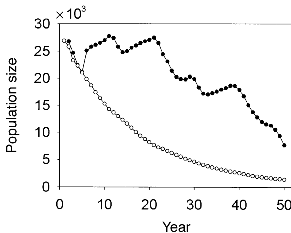
FIG. 3. Predicted population trajectories for Sarracenia purpurea population at Molly Bog (Vermont, USA) using autoregressive (solid circles) and ordinary least-squares (open circles) models for forecasting nitrogen deposition series. For the autoregressive model (Eq. 2), the N time series is modeled with the best-fit coefficients a = 0.0 , b = 0.978 . For the ordinary least-squares model (Eq. 3), the best-fit coefficients were a = 0.477 and b = -0.001 .
