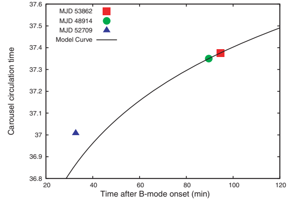
Figure 4. \hat{P}_3 versus the time after ‘B’-mode onset of the three known occurrences of sidebands in B0943+10, along with a model curve representing the relationship established in Paper IV: t = 1.826 \times 10^{-32} \exp[2.077 \hat{P}_3] . There is no discernible relation between the sideband occurrence and the evolution of the ‘B’ mode. The time positions of the MJD 48914 and 53862 observations are calculated from \hat{P}_3 , and should be considered estimations; significant deviation from the model curve is expected, but not plotted here.
