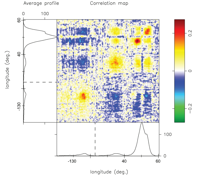
Figure 9. Cross-correlation map of the MJD 53780 PS with itself at a delay of 2 P_1 calculated over the entire 2077 pulses, including both modes. The main panel shows the correlation between different longitudes as marked by the profiles in both the side and bottom panels. The leading and trailing edges of the MP are positively correlated with each other and the PC (and negatively correlated with the IP), whereas the centre of MP correlates with neither. This strongly indicates that the MP has a three-zone emission structure, although this is not fully clear from its average profile. The ordinate is delayed with respect to the abscissa, and the positive (negative) delay maps are shown below (above) the diagonal; these two maps are virtually identical, indicating correlations that are time-reversible. The 3\sigma error in the correlations is about 6 per cent.
