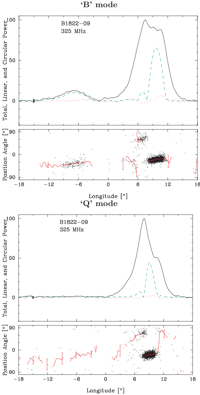
Figure 8. Average profiles and polarization histograms of the PC and MP of B1822-09 during its ‘B’ (pulse #s 1200–1455) and ‘Q’ (#s 200–770) modes, in Fig. 7, respectively. ‘B’ mode (top): here the highly linearly polarized PC ‘turns on,’ and its nearly flat PPA traverse is remarkable. Accounting for the 90° OPM ‘jump,’ the MP PPA is also essentially flat, suggesting a nearly central sightline traverse. ‘Q’ mode (bottom): the conal components flanking the central MP feature have reduced intensity, so the profile is narrower. PC emission is still faintly visible, along with a trace of its linear polarization. The quantities plotted are the same as in Fig. 5.
