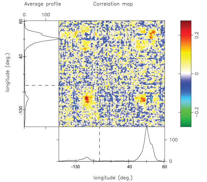
Figure 12. Cross-correlations of the PS with itself at a delay of 2P_1 , calculated over pulses 221–750 of the ‘Q’ mode-only MJD 53780 observation. Here, we see a strong correlation of the IP with itself as well as a significant correlation of the delayed IP with the leading region of the MP profile, but not the reverse. Note also that it is a trailing region of the IP that is modulated, but a long leading region precedes it. The 3\sigma error in the correlations is about 13 per cent. See Fig. 9 for details.
