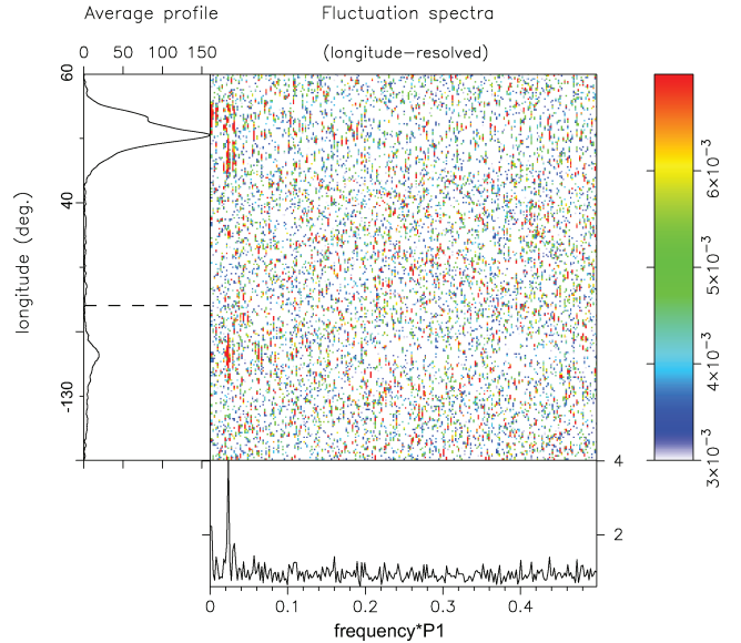
Figure 10. LRF spectra of pulsar B1822–09’s ‘Q’ mode, averaged over pulses 221–750 of the MJD 53780 observation, using a 512 point FFT. The MP is at the top of the left-hand panel, the PC in the centre, and the IP at the bottom. A strong feature at 0.023 \text{ c } P_1^{-1} , corresponding to a P_3 of about 43P_1 , modulates both the MP and the IP, while the weak PC displays no discernible modulation.
