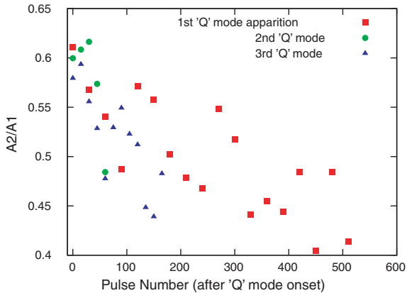
Figure 14. Changes in the trailing (A2) to peak (A1) amplitude ratio in the B1822–09 MP profile following ‘Q’-mode onset. The amplitudes are measured from 30 pulse averages of the MJD 53780 observation. A1 is measured at the peak of the profile and A2 as the intensity \sim 3^\circ later, at the peak of the trailing component.
