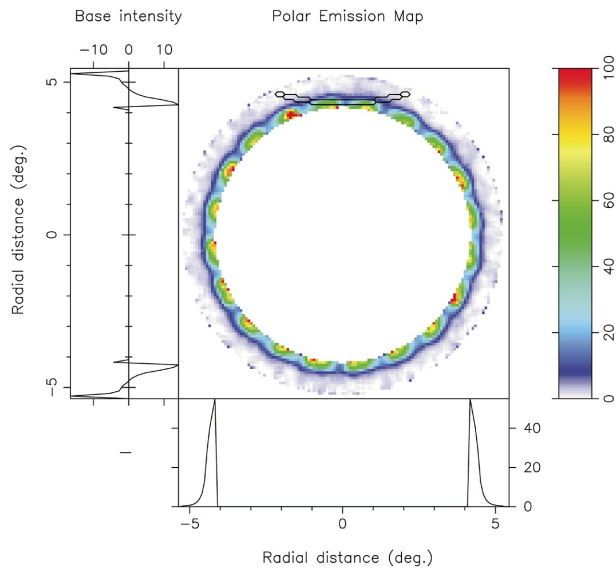
Figure 10. An image of the accessible emission zone reconstructed using the ‘cartographic’ transform as defined by equations (5)–(9). This image is based on the observed ‘B’-mode sequence of 816 pulses. The image or polar map is projected on to the polar cap shown in the main panel, with the ‘closer’ rotational axis at the top of the diagram. The bottom and the side panels show the average- and the ‘base’-intensity profiles, respectively, as functions of the angular distance from the magnetic axis (i.e. magnetic colatitude). Contours indicate the sightline path at the top of the diagram. Here, the star rotates clockwise, causing the sightline to cut the counter-clockwise-rotating sub-beam pattern from left to right.
