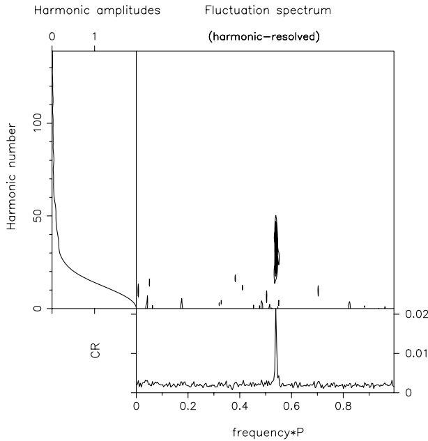
Figure 22. HRF spectrum as in Fig. 4 for the 1972 430-MHz subsequence. Note that the primary modulation feature is at 0.54 \text{ cycle } P_1^{-1} – related as before to the aliased 0.46\text{-cycle } P_1^{-1} feature in the LRF spectrum (not shown). Contours are at intervals of 28 \text{ mJy}^2 up to 198 \text{ mJy}^2 .
