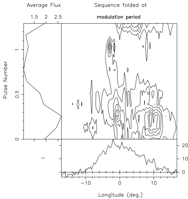
Figure 14. Folded PS corresponding to the 128-pulse ‘Q’-mode subsequence in Fig. 12. The data have been averaged over 10 bins spanning the amplitude-modulation feature at 1.293P_1 cycle -1 . The ‘base’ profile (bottom panel) has been subtracted from the folded sequence (main panel). The modulation is deep and confined to a -2^\circ to +10^\circ longitude range. Contours are at 13-mJy intervals.
