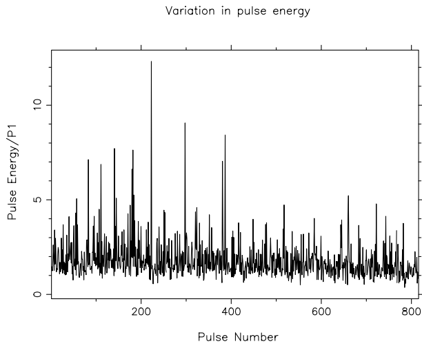
Figure 2. Pulse energy as a function of pulse number of the 816 pulses comprising the ‘B’-mode sequence. Notice the slight secular decrease in intensity and its periodic tendencies, and, most of all, notice that there is not a single ‘null’ pulse!
