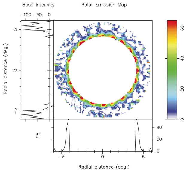
Q43 Figure 23. Polar emission map obtained via the ‘cartographic’ transform for the 1972 430-MHz observation as in Fig. 10. The map is smoothed with a circular 8-pixel-area window to reduce the noise in its peripheral regions.
