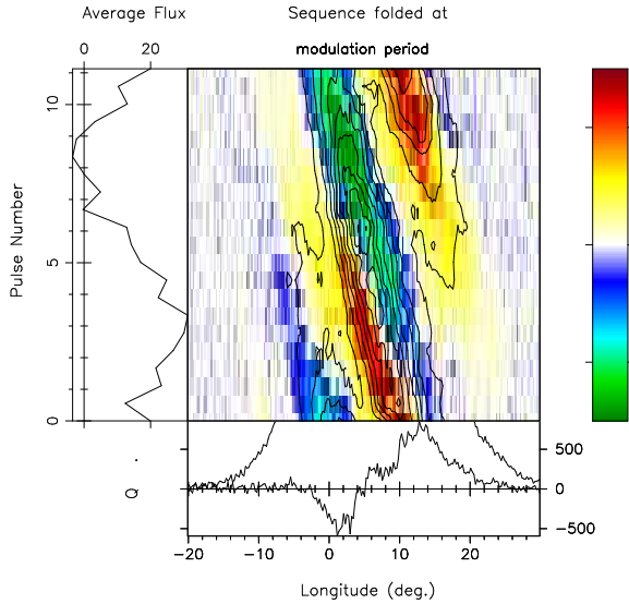
Figure 2. Folded 328-MHz driftband (top left) showing the total power (contours) and the modal polarization (colour-intensity coded) in terms of the rotated Stokes parameter Q' (see Paper 0 for details). The two OPMs are coded positive and negative, and close inspection shows that the total power driftband is canted with respect to the two modal overlapping driftbands. (top right) A display of the total power modulation phase, with the profile and the modulated power in the top panel and the phase in the lower one. (bottom right) Polarized profile of the same pulse sequence. The overall depolarization is striking, and one can see that the two regions of modal polarization overlap more in the leading region than the trailing.
