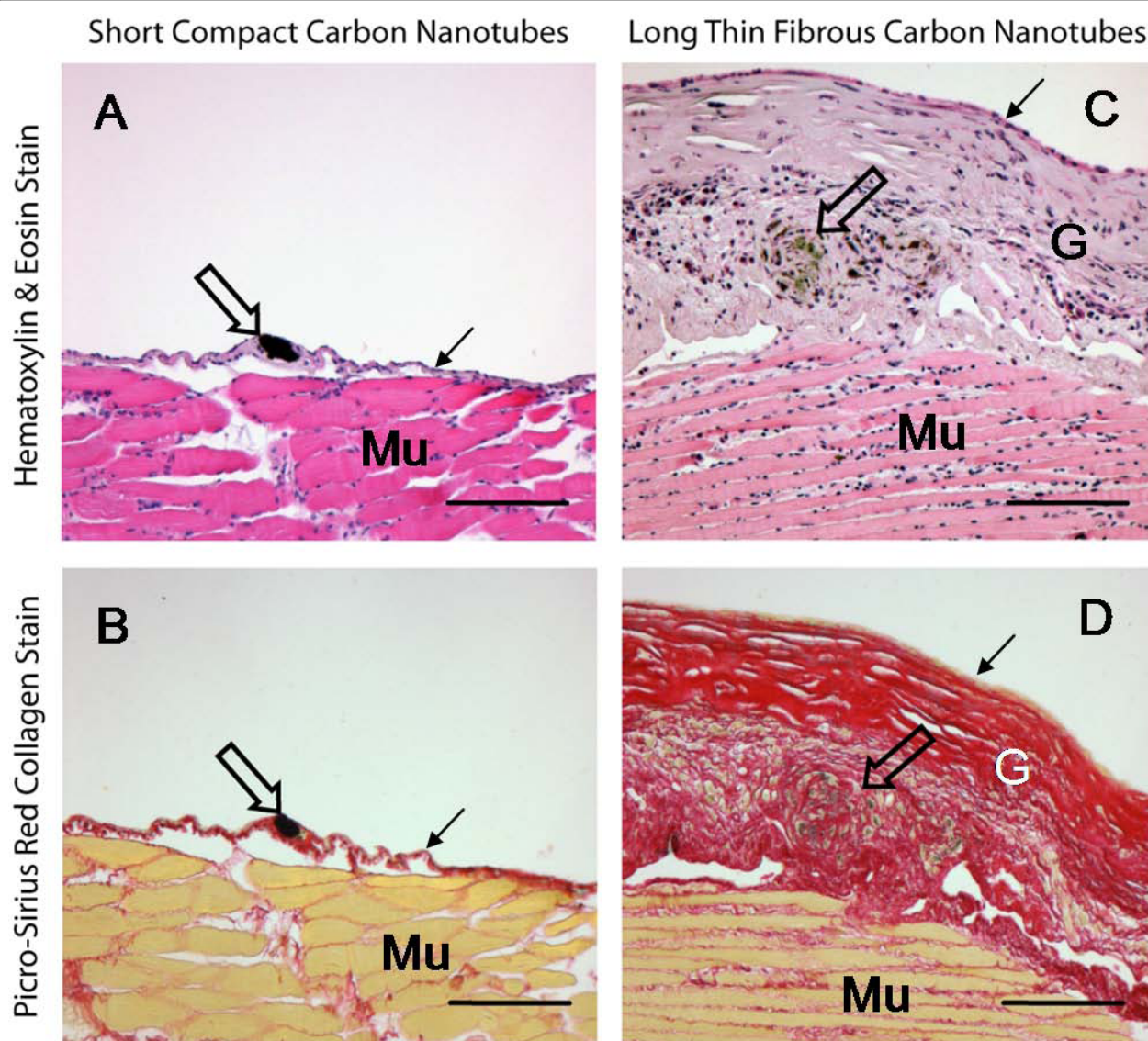
Figure 6 Lesions on the peritoneal face of the diaphragm after intra-peritoneal injection of 2 forms of carbon nanotube differing in aspect ratio. The figure shows sections through the peritoneal aspect of the diaphragm of C57BL/6 mice 6 months after intra-peritoneal injection of 10 µg of two separate forms of multi-walled carbon nanotube (CNT). Sections are stained with Haematoxylin & Eosin (panels A and C) or Picro-sirius red stain which stains collagen bright red (panels B and D). Mu = Muscle of diaphragm; G = granuloma; small arrows = mesothelium; large arrows = carbon nanotubes. C and D show a large granuloma sitting atop the muscle layer, caused by the presence of CNT in the form of long fibres (open arrows). A and B show the contrasting response to CNT in the form of tightly bound dense spherical aggregates (open arrows) which produces minimal tissue reaction. All images are taken at ×100 magnification bar = 100 µm.
