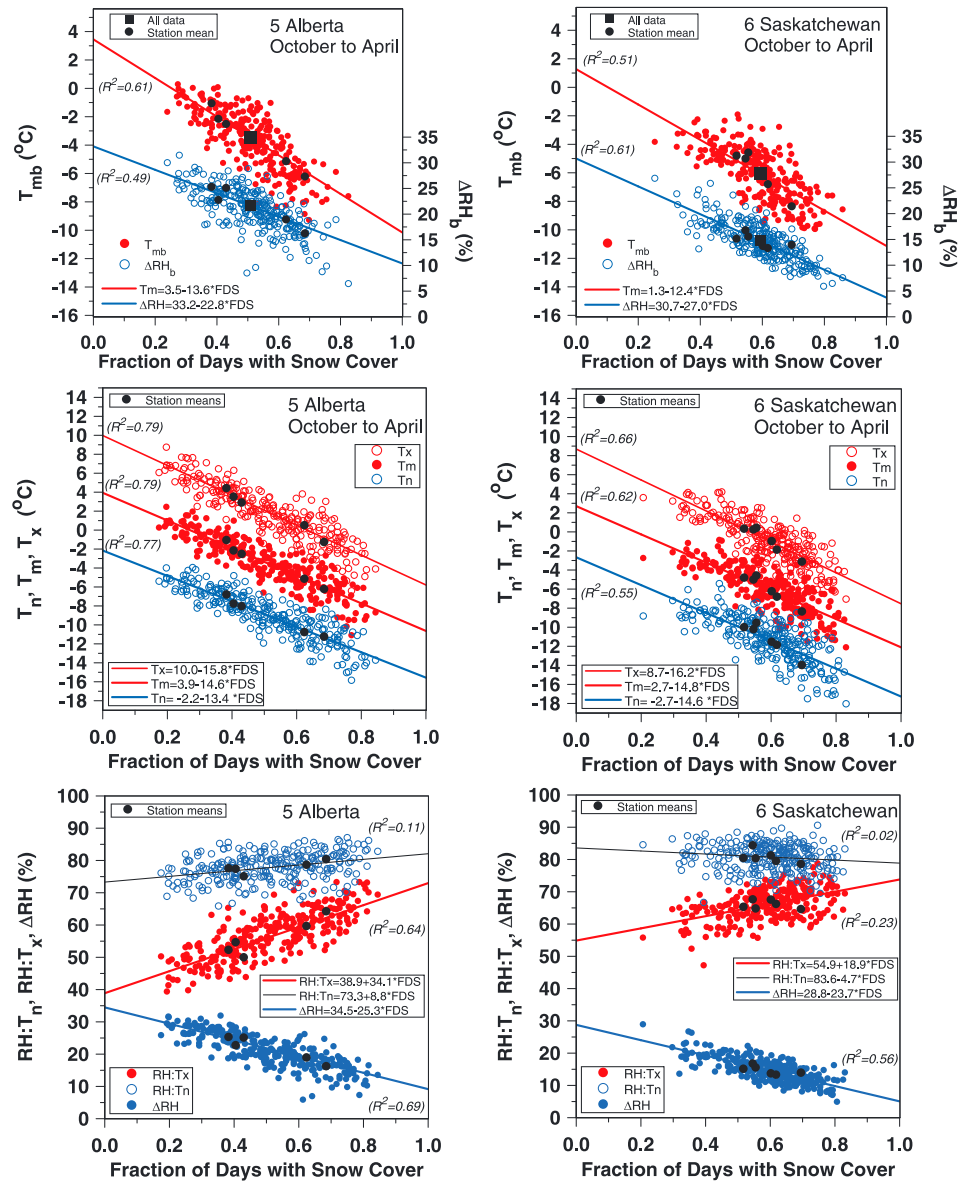
Figure 6. T_{mb} and \Delta RH_b plotted against fraction of days with (top row) snow cover, (middle row) T_x , T_m , and T_n , and (bottom row) RH:T_n , RH:T_x , and \Delta RH against fraction of days with snow cover.
