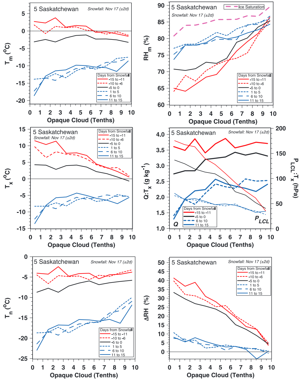
Figure 7. Coupling between cloud cover and surface climate across fall-winter snow transitions.
