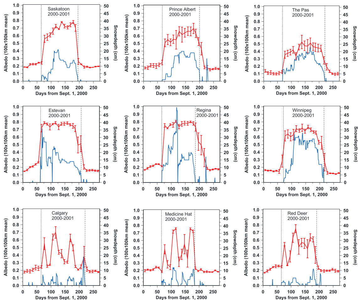
Figure 9. Comparison of station snow depths (blue) with 100 \times 100 km MODIS albedo (red) from September to May.
