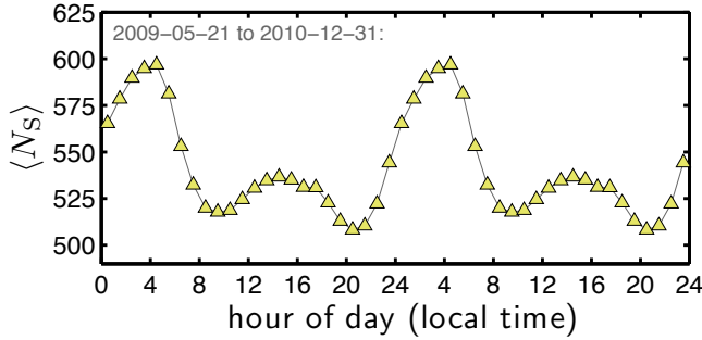
FIG. 13: Average Simpson lexical size N_S for time of day, corrected according to local time, and computed for each day with outlier days removed, and then averaged across days. See also Fig. S4 in Supplementary Information for a demonstration of the robustness of the form of N_S throughout the day under alternate averaging schemes.
