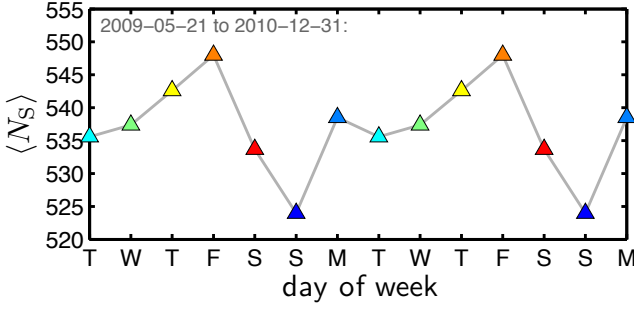
FIG. 9: Simpson lexical size as a function of day of the week. We compute N_S for individual dates Fig. 3B, again excluding dates shown in Fig. 3A, and then average these values. (See also Fig. S3 for the effects of alternate approaches.)
