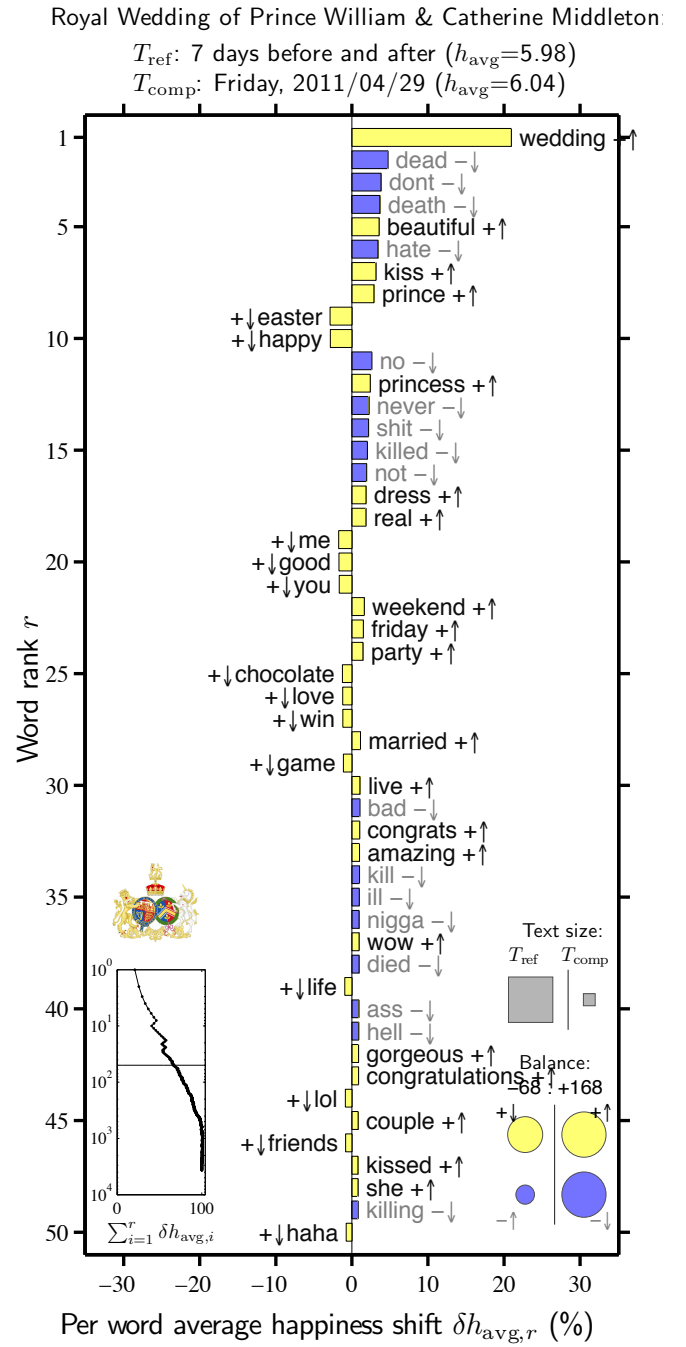
FIG. S44: Word shift graph for Royal Wedding of Prince William & Catherine Middleton, 2011/04/29, relative to 7 days before and 7 days after combined.
