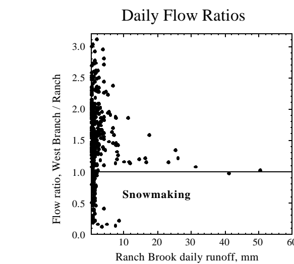
Figure 6: Ratio of West Branch to Ranch Brook average daily flow vs. Ranch Brook average daily flow (WY 2001).
