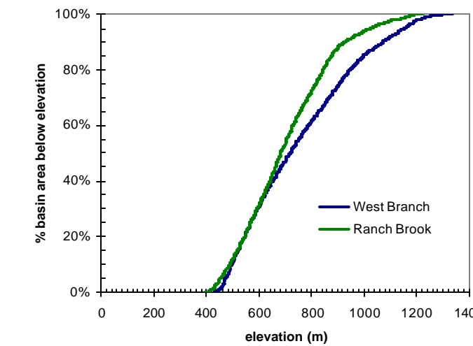
Figure 2: Basin hypsometry
