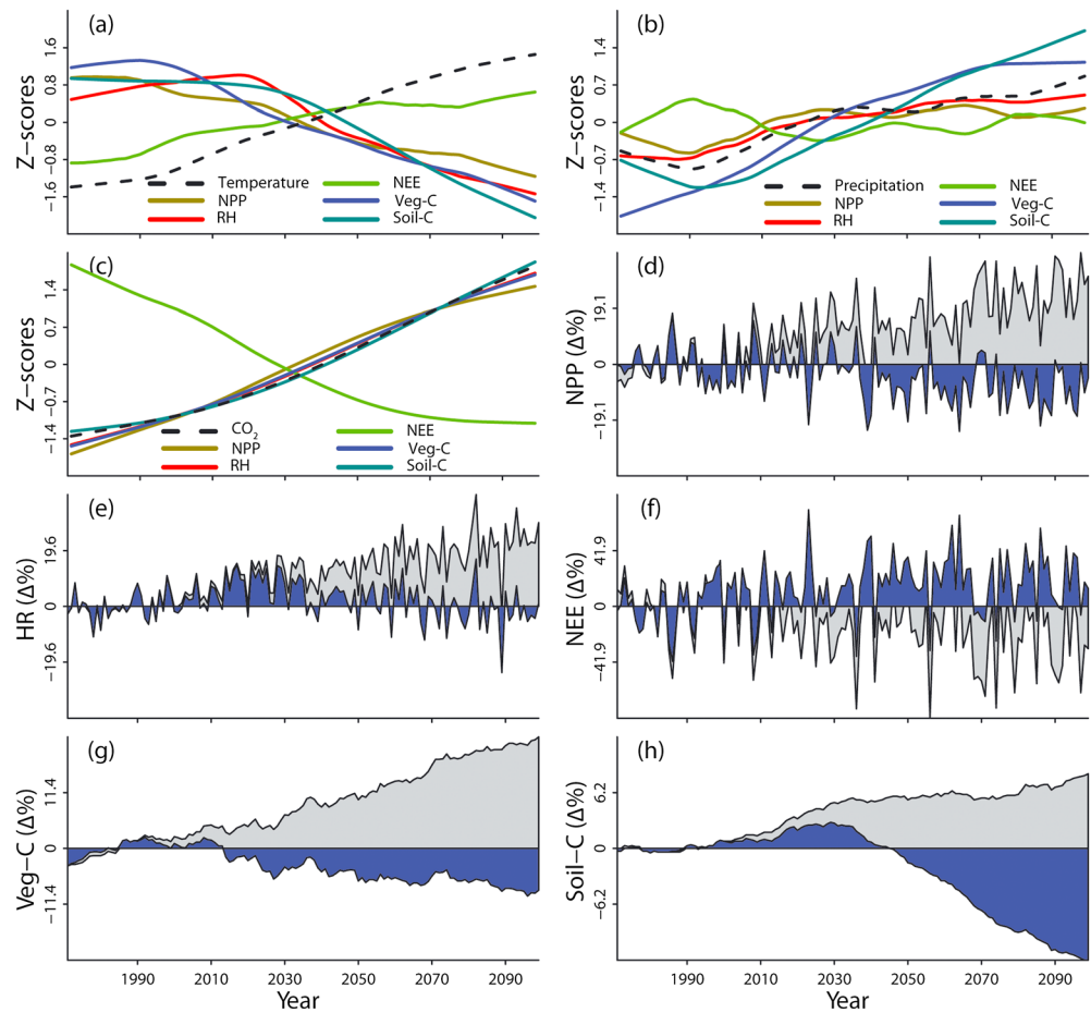
Figure 4. Effects of variation in (a) annual mean temperature, (b) total precipitation, and (c) atmospheric CO 2 concentration alone on C dynamics during 1971–2099. (d–h) Comparisons of simulated C dynamics between scenario with (gray) and without (blue) considering elevation of CO 2 levels under the HadCM3 A1B scenario. Data shown in Figures 4d–4h are percent changes relative to the baseline conditions.
