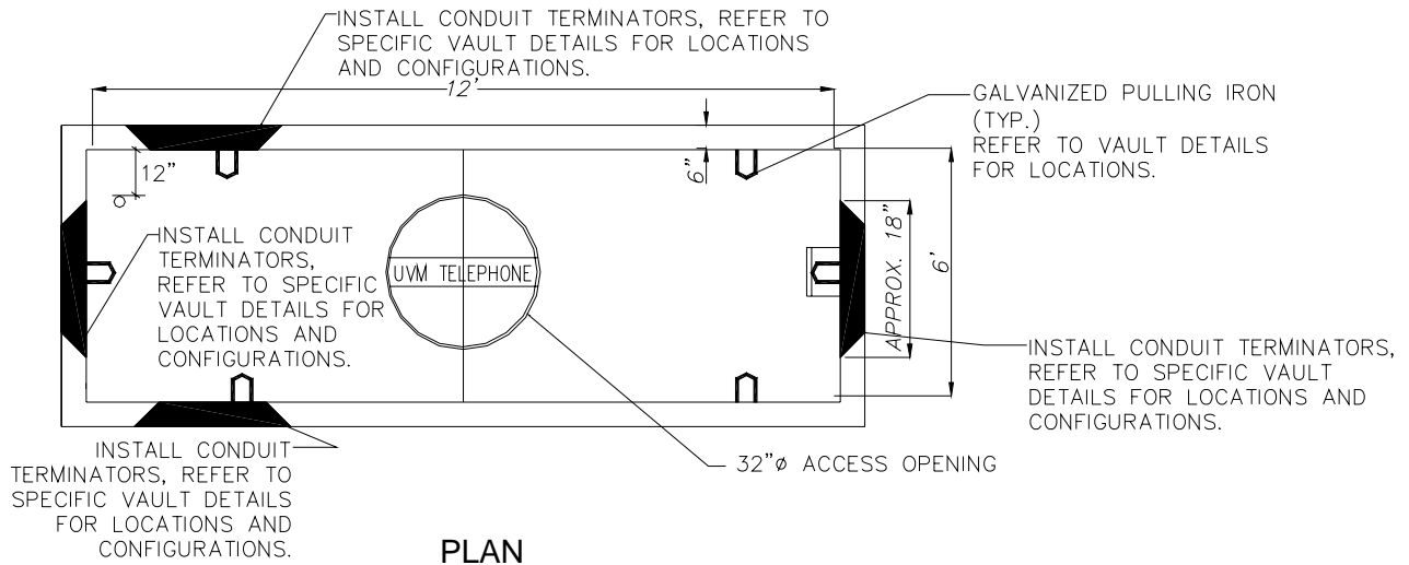
Detail #1 Typical Precast Vault Detail
