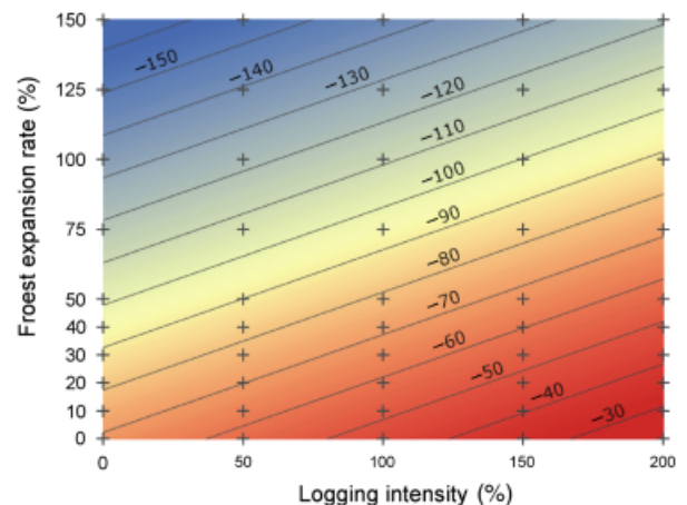
Fig. 6 Total carbon sink strength [ \text{Tg C} ] between 2008 and 2100 for different scenarios of logging intensity ( 100\% = 5000 \text{ ha yr}^{-1} ) and forest expansion ( 100\% = all currently unused farmland \sim 728\,000 \text{ ha} ). Crosshairs mark modeled scenarios; isolines denote identical sink strength across different scenarios.
