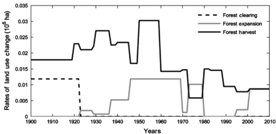
Fig. 3 Rates of permanent forest clearing, forest harvesting, and forest expansion for the time period 1900–2007 used as input data for the carbon bookkeeping model.
