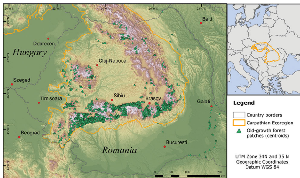
Figure 1 Study area in the Carpathian Mountains in Romania including the distribution of old-growth forest patches (Source: SRTM digital elevation model, see URL http://srtm.csi.cgiar.org ; ESRI Data and Maps Kit, see URL http://www.esri.com/data/data-maps ).
