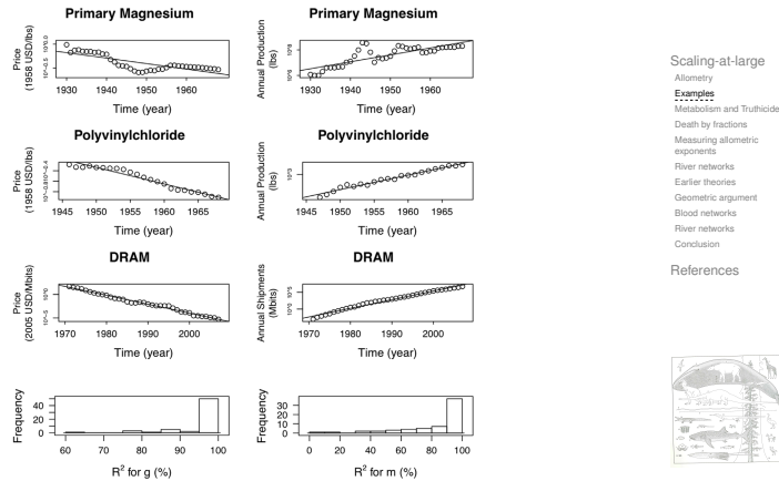
Figure 3. Three examples showing the logarithm of price as a function of time in the left column and the logarithm of production as a function of time in the right column, based on industry-wide data. We have chosen these examples to be representative. The top row contains an example with one of the worst fits, the second row an example with an intermediate goodness of fit, and the third row one of the best examples. The fourth row of the figure shows histograms of R^2 values for fitting g and m for the 62 datasets.
