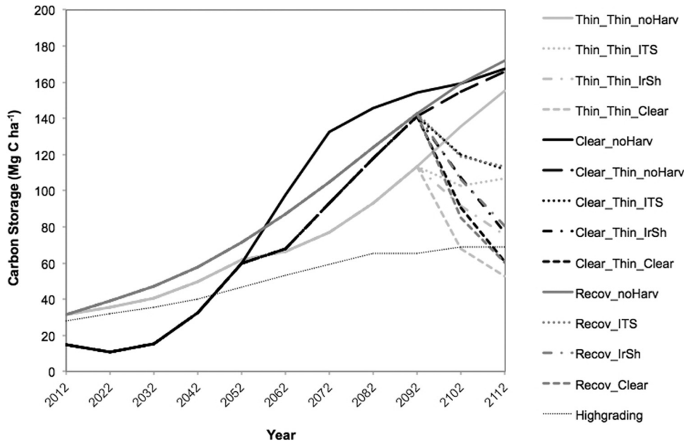
Fig. 4. Average carbon stores over 100 years in live tree, dead tree, and harvested wood product (HWP) carbon pools.
