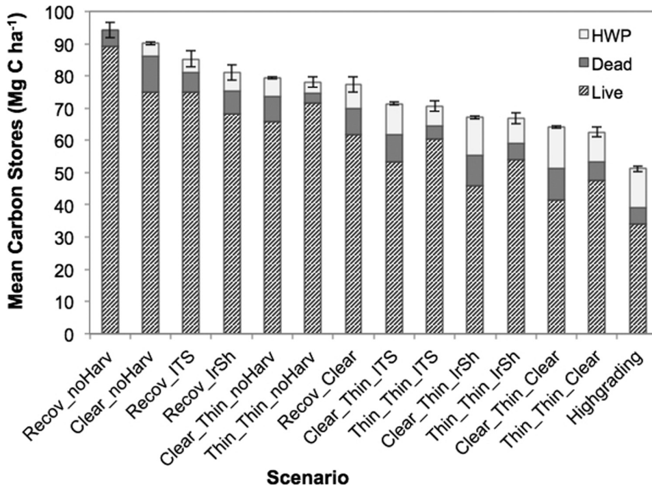
Fig. 4. Average carbon stores over 100 years in live tree, dead tree, and harvested wood product (HWP) carbon pools.
