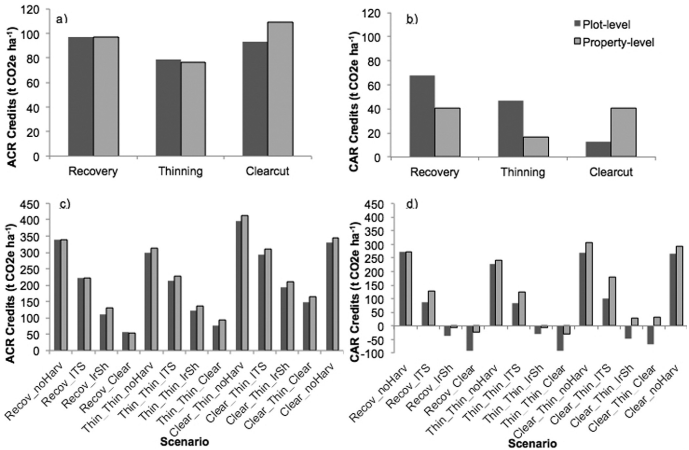
Fig. 6. Comparison of plot-level versus property-level carbon credit calculations after (a) 40 years under ACR, (b) 40 years under CAR, (c) 100 years under ACR, and (d) 100 years under CAR.
