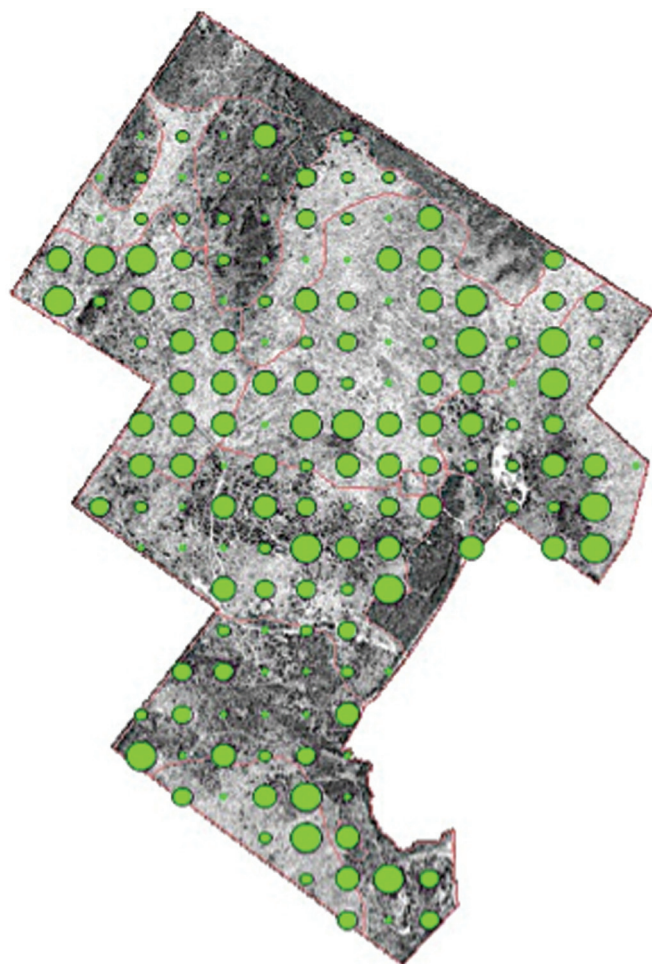
Fig. 1. Variability in average carbon stores on the Victory property as calculated in the starting year, 2012. Circle sizes represent plot-level estimates of CO 2 e in tonnes per hectare that is stored in aboveground live trees. Estimates are spatially accurate at the stand level.
