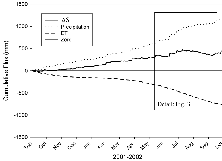
Fig. 2. Cumulative water balance between 1 September, 2001 and 1 October, 2002. Daily precipitation, evapotranspiration, and change in storage of the peat system are shown over the sample period.
