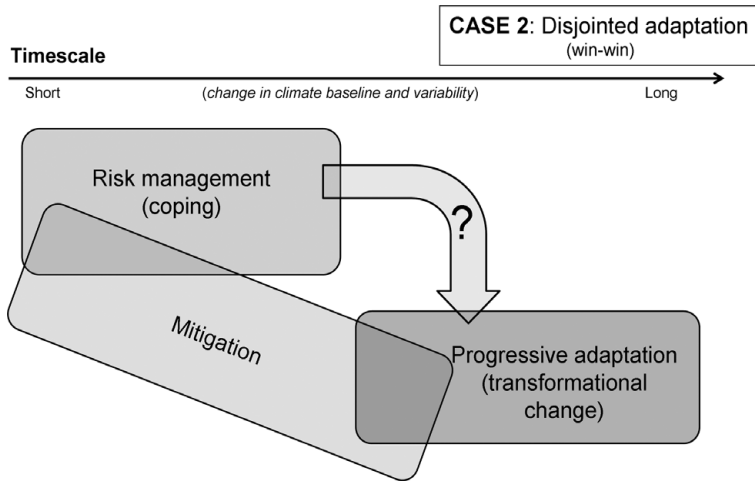
Figure 4. The first case of disjointed adaptation with opportunities of transitioning systems through mitigation actions.
