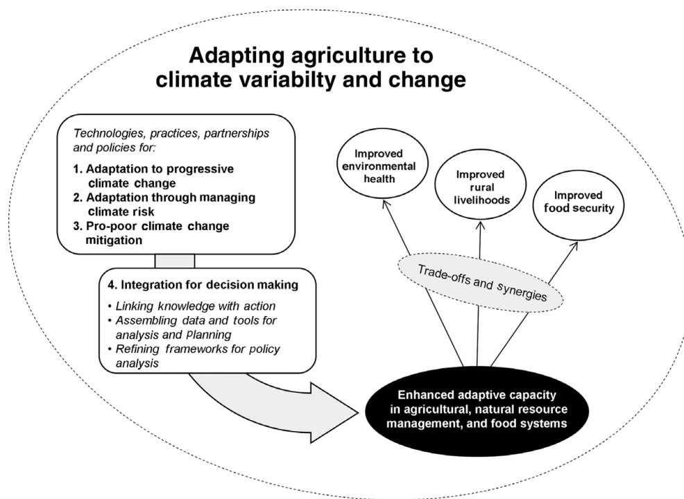
Figure 1. CCAFS framework for adaptation and mitigation research.
