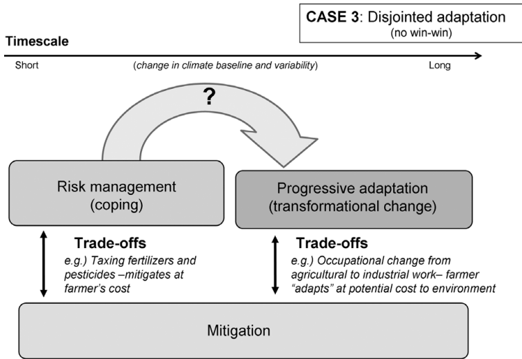
Figure 5. The second case of disjointed adaptation where all potential interventions require careful analysis of trade-offs.
