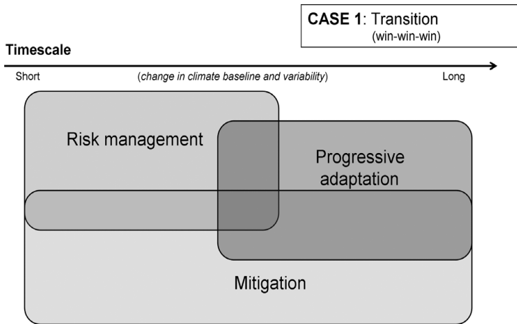
Figure 3. The triple win transition case, whereby risk management, progressive adaptation and mitigation all provide synergies.
