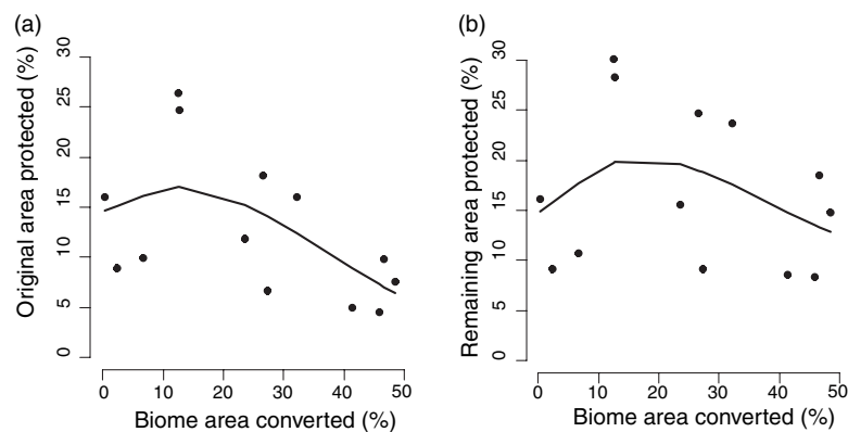
Figure 2 (a) Cubic spline (3 d.f.) fit to relationship between per cent area converted and per cent area protected for the 13 terrestrial biomes of the world. \text{Adj. } R^2 = 0.6 from general additive model (GAM). (b) Cubic spline (3 d.f.) fit to relationship between per cent area converted and per cent of remaining area protected data for each terrestrial biome. \text{Adj. } R^2 = 0.10 from GAM. Estimates of per cent of remaining area protected were calculated by dividing the total protected area in each biome by the area of non-converted land cover in each biome. Although this relationship appears less pronounced, biomes with intermediate levels of habitat conversion still have greater levels of habitat protection, while biomes with very low or very high habitat conversion have less.
